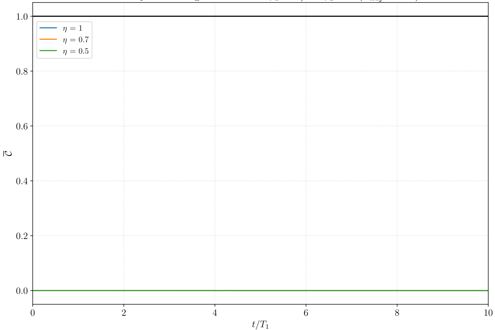
Heterodyne: Average \bar{\mathcal{C}} over time \phi_1 = \pi/2 \phi_2 = 0 ( n_{\text{traj}} = 100 )
