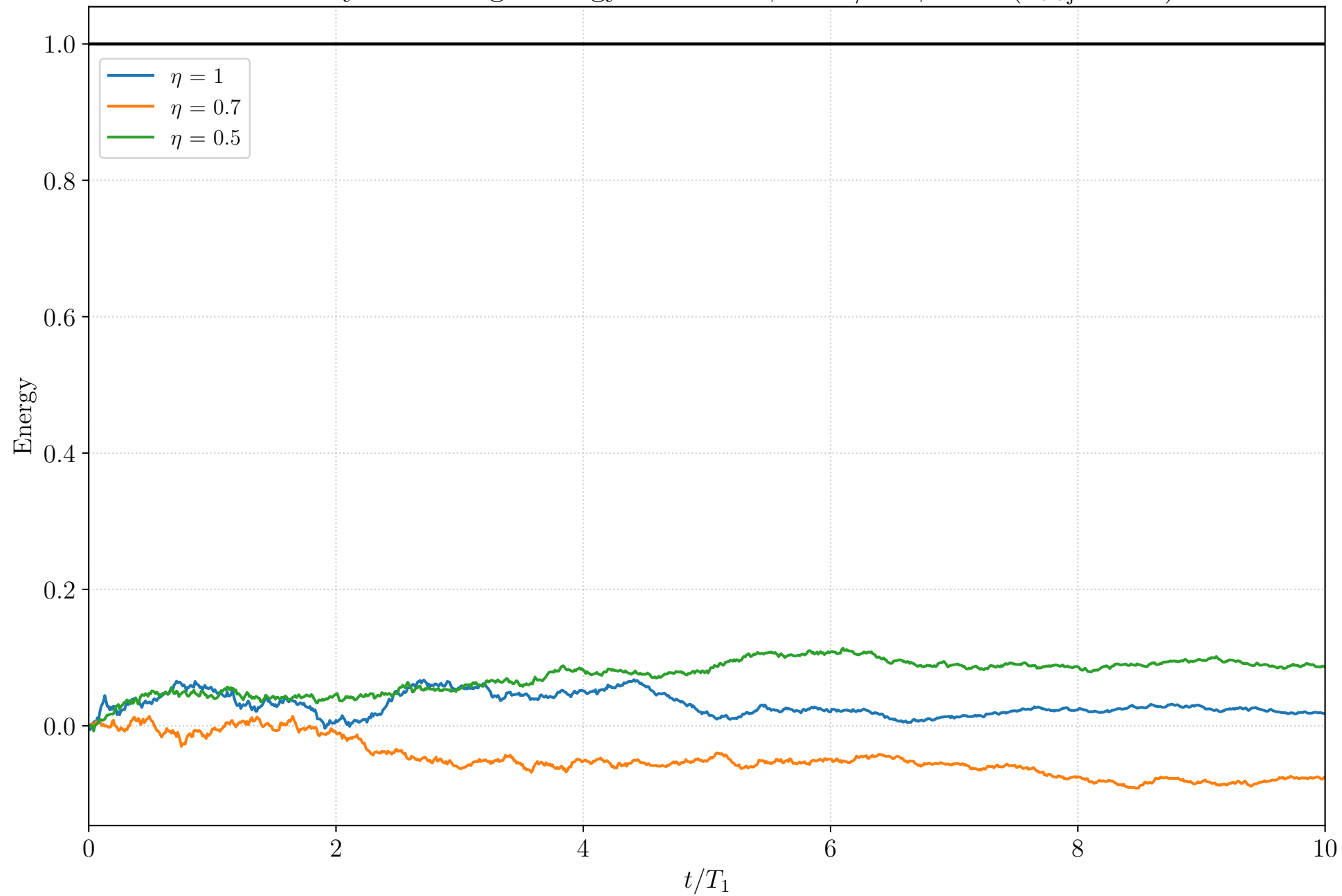
Heterodyne: Average Energy over time \phi_1 = \pi/2 \phi_2 = 0 ( n_{\text{traj}} = 100 )
