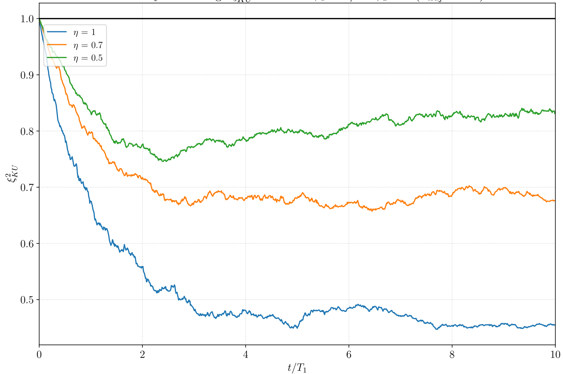
Heterodyne: Average \xi_{KU}^2 over time \phi_1 = \pi/2 \phi_2 = 0 ( n_{\text{traj}} = 100 )
