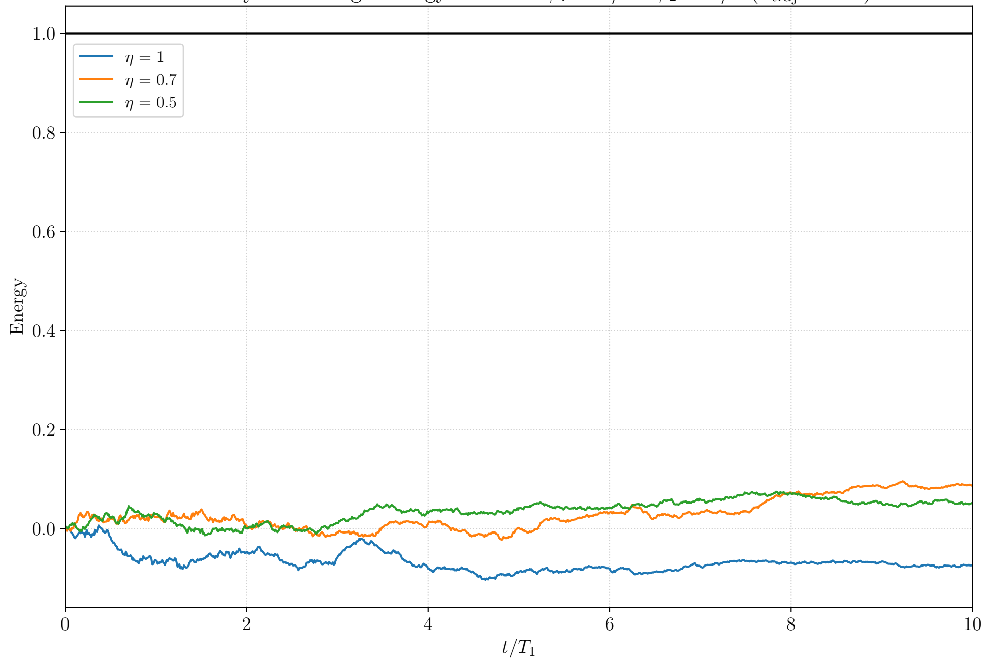
Heterodyne: Average Energy over time \phi_1 = \pi/2 \phi_2 = \pi/2 ( n_{\text{traj}} = 100 )
