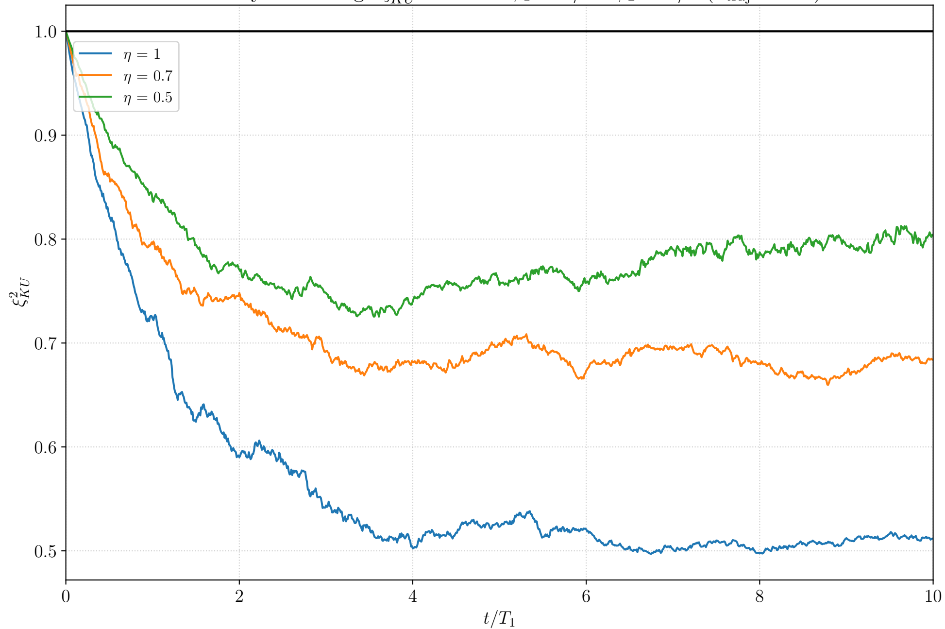
Heterodyne: Average \xi_{KU}^2 over time \phi_1 = \pi/2 \phi_2 = \pi/2 ( n_{\text{traj}} = 100 )
