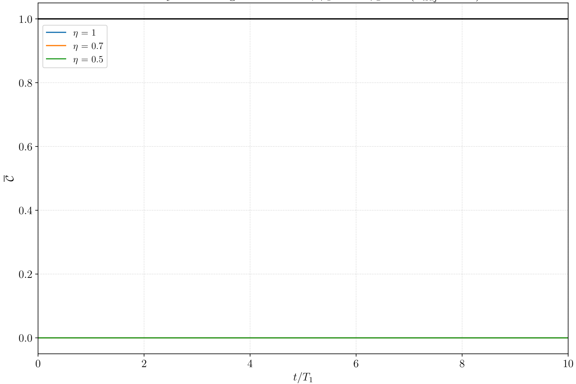
Homodyne: Average \bar{\mathcal{C}} over time, \phi_1 = 0 \phi_2 = 0 ( n_{\text{traj}} = 100 )
