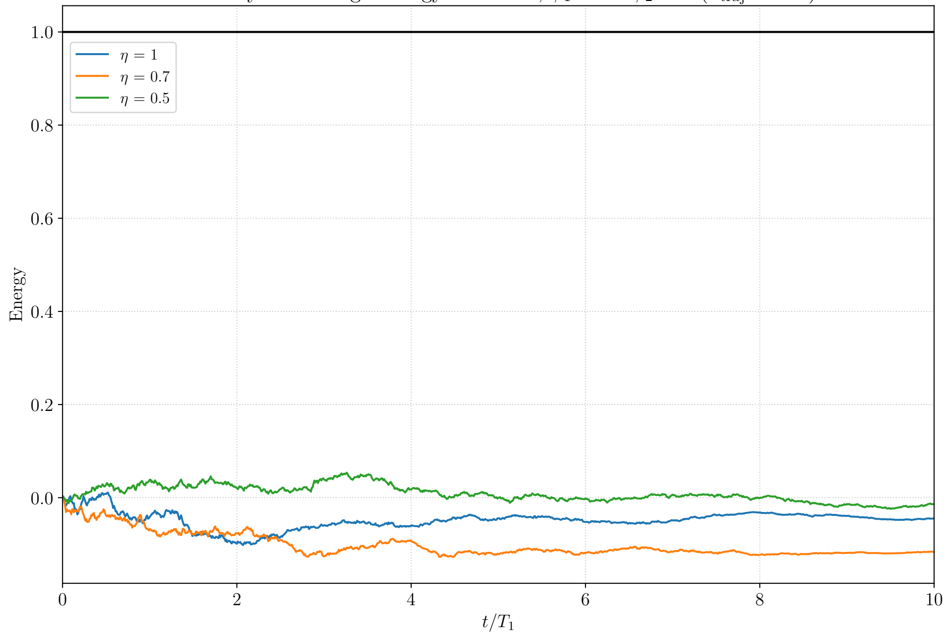
Homodyne: Average Energy over time, \phi_1 = 0 \phi_2 = 0 ( n_{\text{traj}} = 100 )
