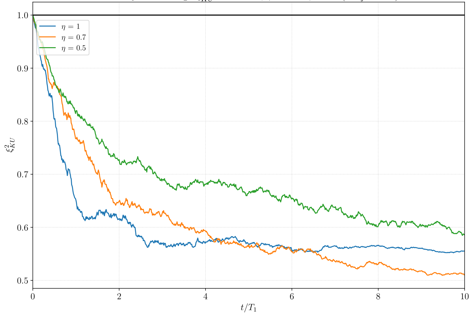
Homodyne: Average \xi_{KU}^2 over time, \phi_1 = 0 \phi_2 = 0 ( n_{\text{traj}} = 100 )
