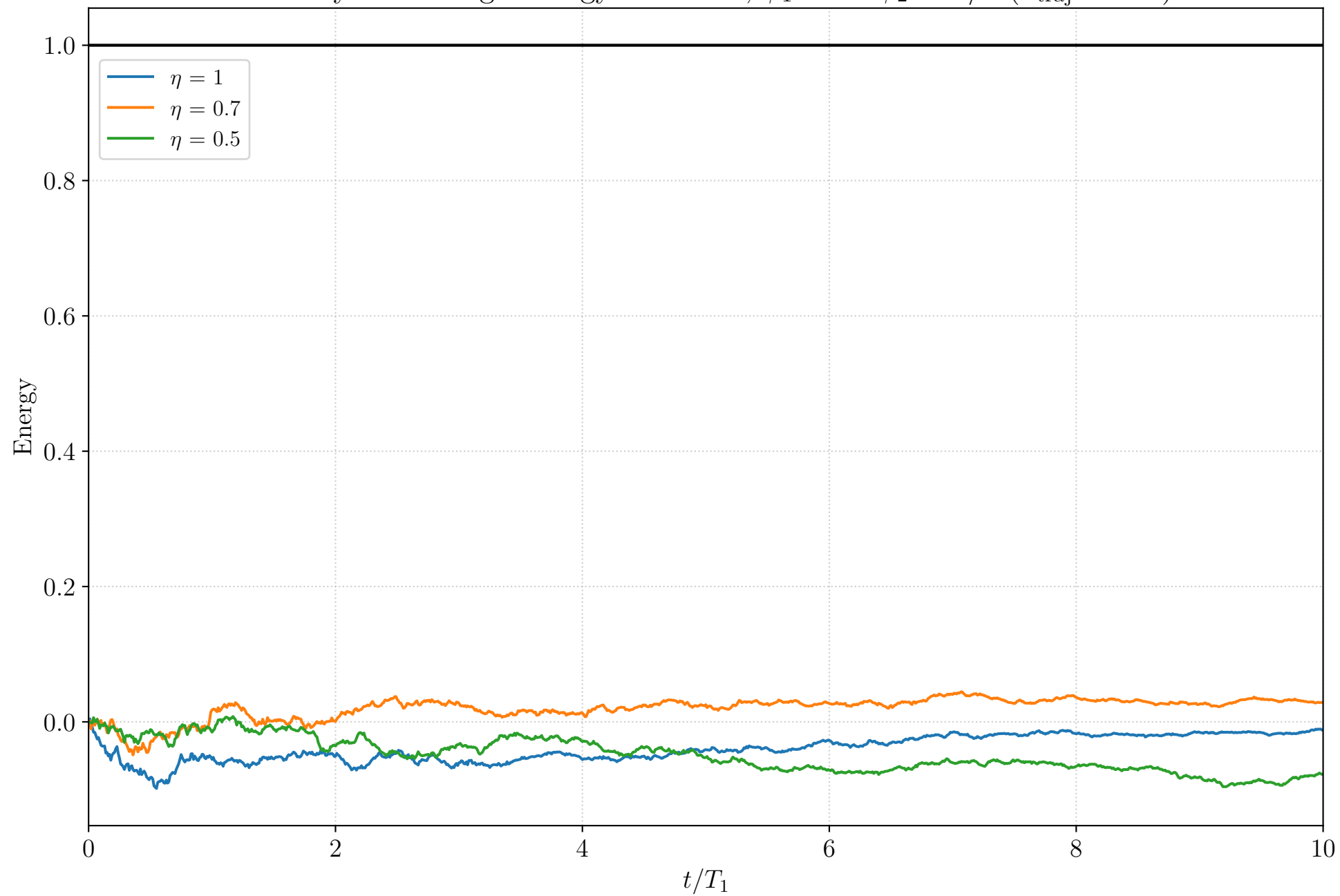
Homodyne: Average Energy over time, \phi_1 = 0 \phi_2 = \pi/2 ( n_{\text{traj}} = 100 )
