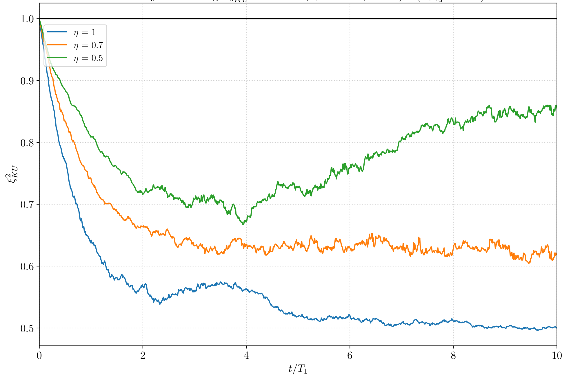
Homodyne: Average \xi_{KU}^2 over time, \phi_1 = 0 \phi_2 = \pi/2 ( n_{\text{traj}} = 100 )
