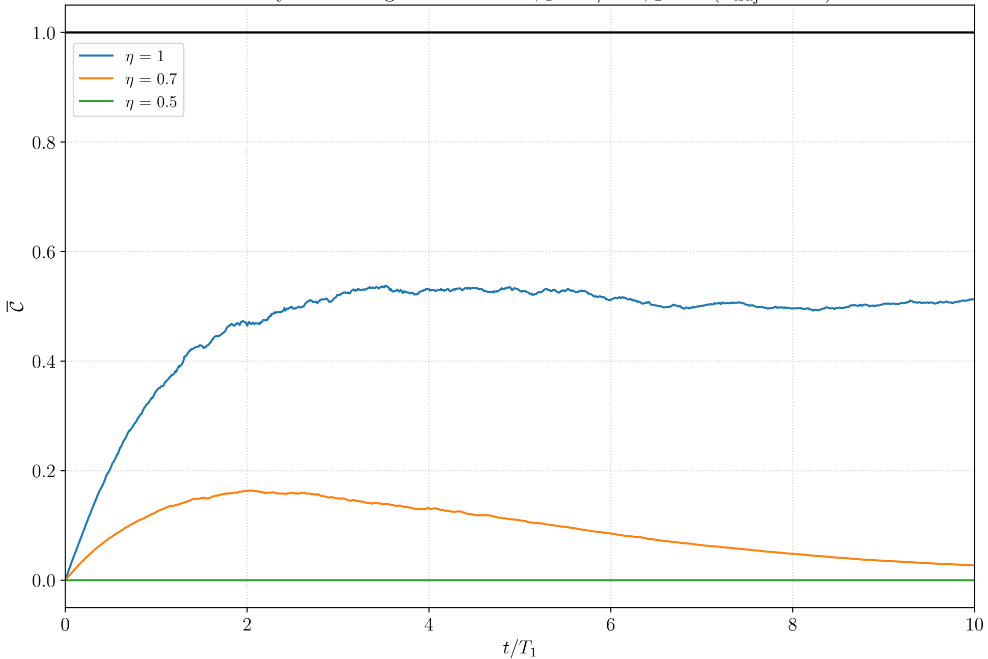
Homodyne: Average \bar{\mathcal{C}} over time \phi_1 = \pi/2 \phi_2 = 0 ( n_{\text{traj}} = 100 )
