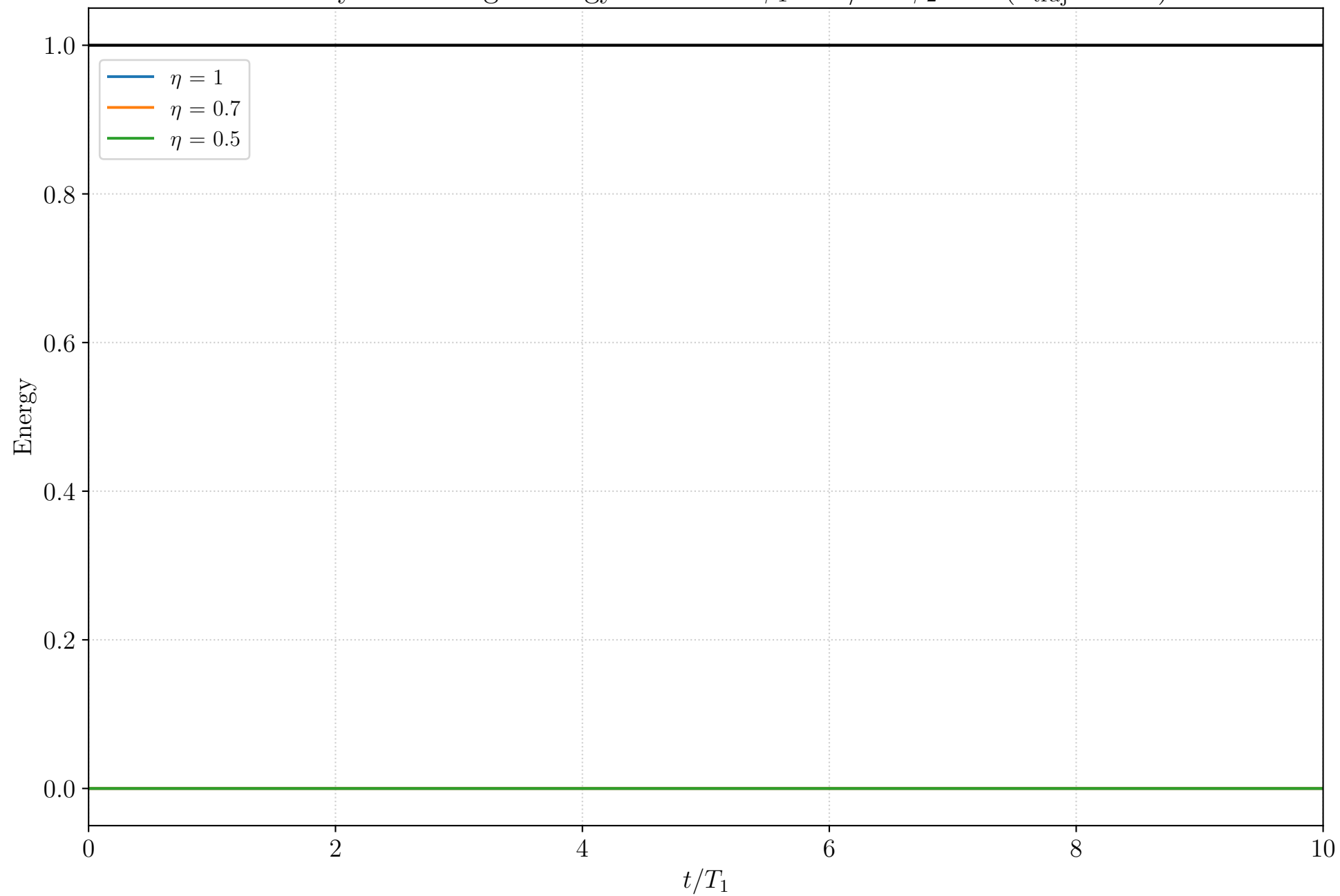
Homodyne: Average Energy over time \phi_1 = \pi/2 \phi_2 = 0 ( n_{\text{traj}} = 100 )
