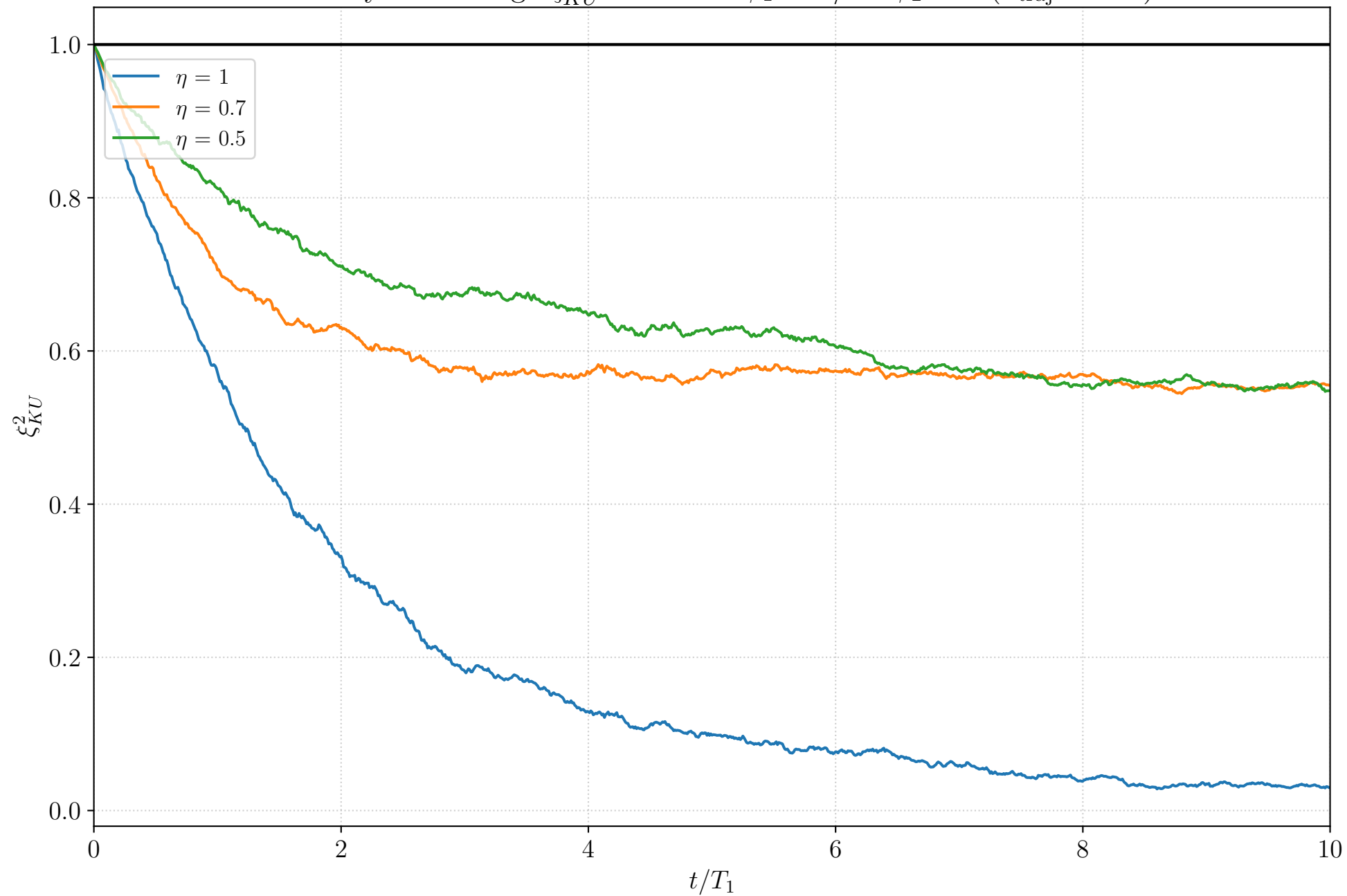
Homodyne: Average \xi_{KU}^2 over time \phi_1 = \pi/2 \phi_2 = 0 ( n_{\text{traj}} = 100 )
