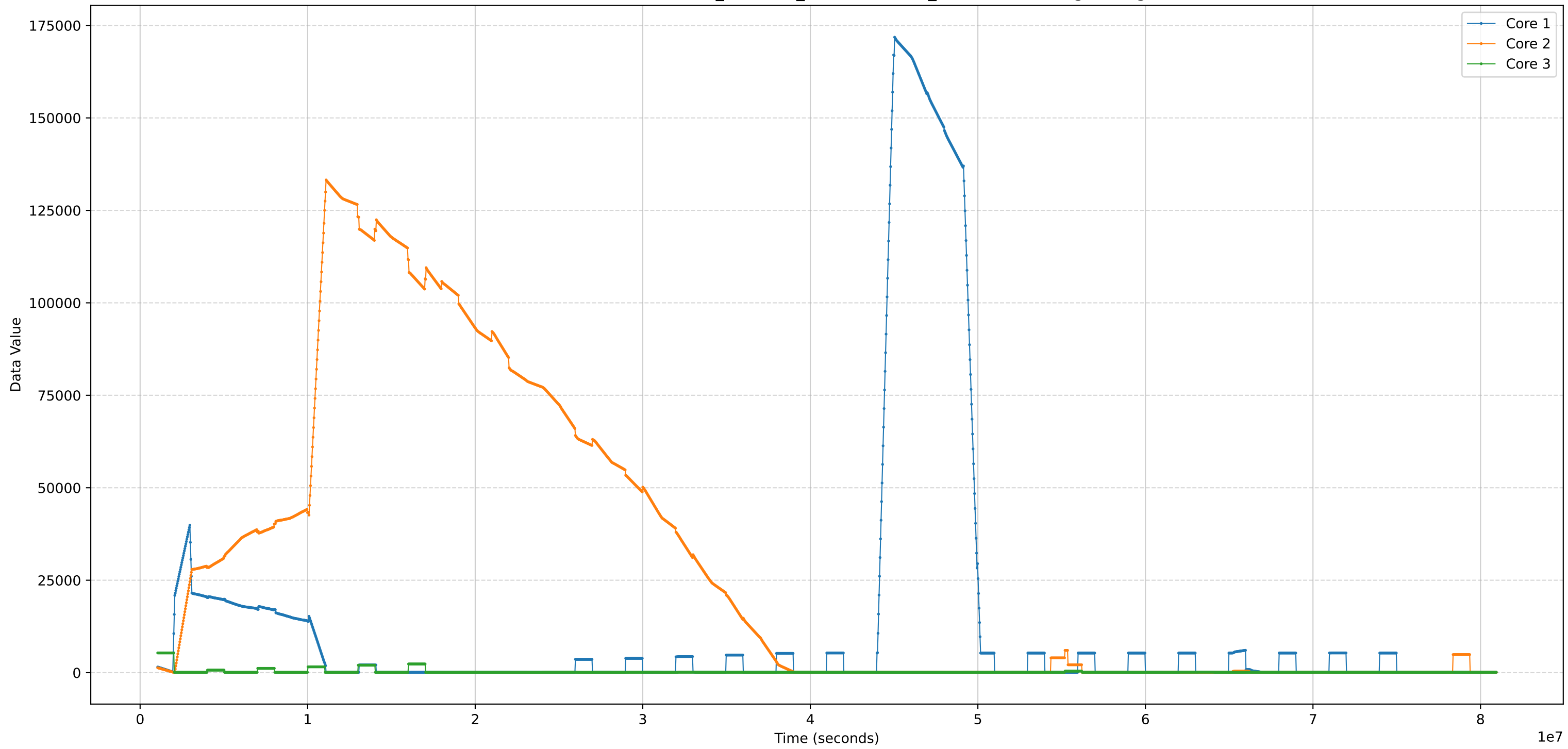
Benchmark Data - ATOMIC_MEMORY_INSTRUCTIONS_RETIRED - Moving average
