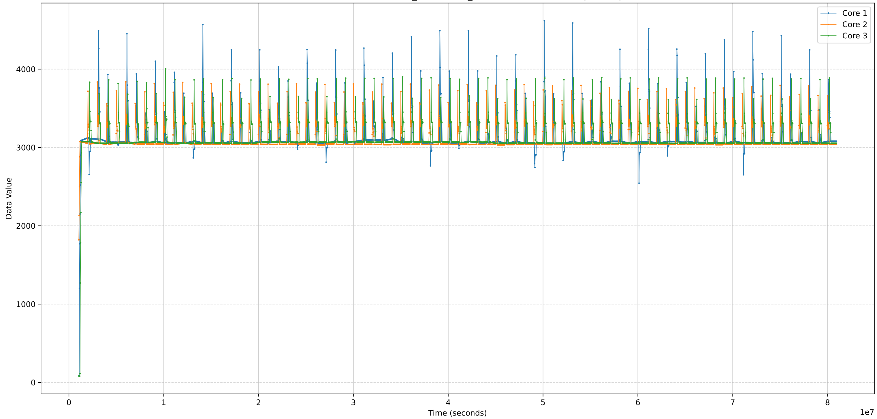
Benchmark Data - BRANCH_DIRECTION_MISPREDICTION - Moving average
