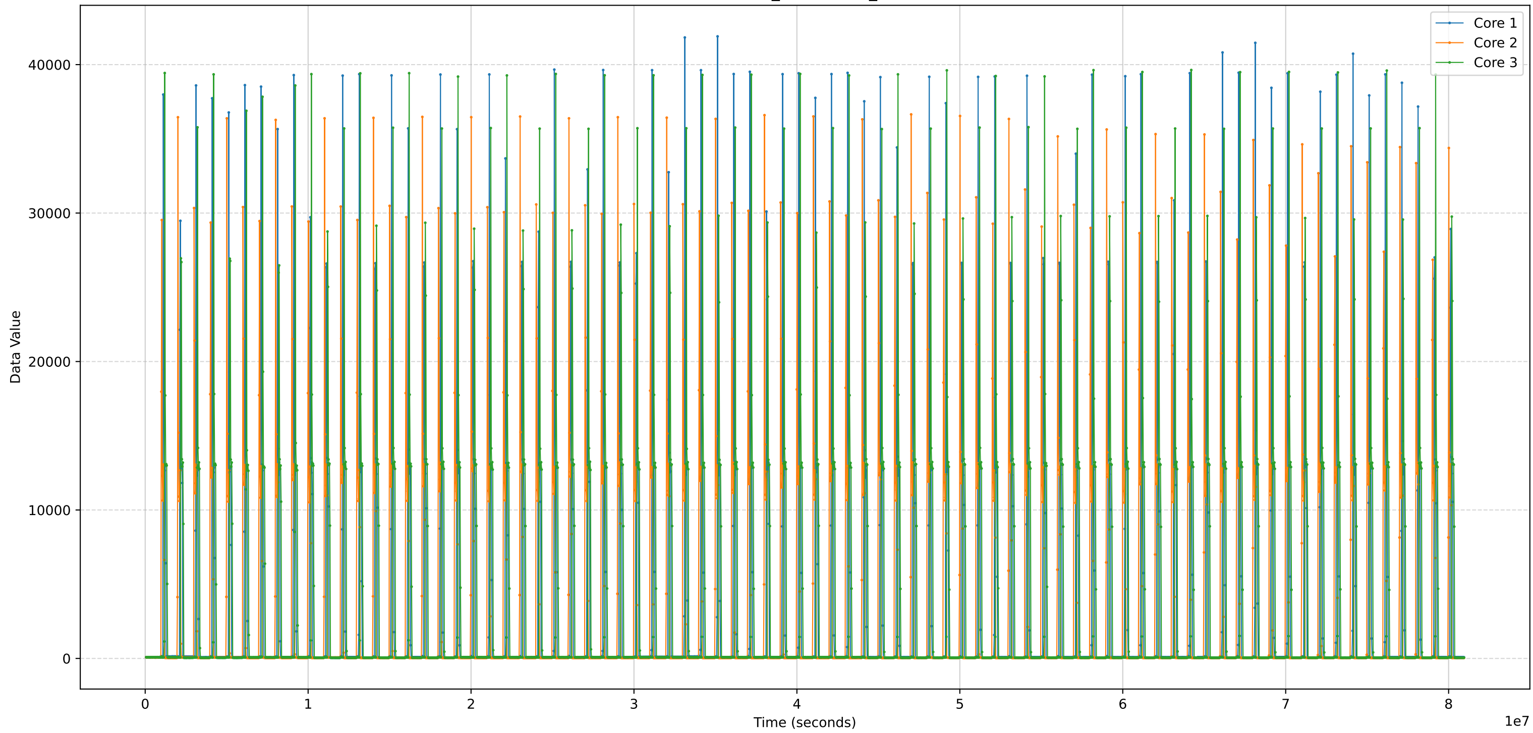
Benchmark Data - BRANCH_DIRECTION_MISPREDICTION - Rate
