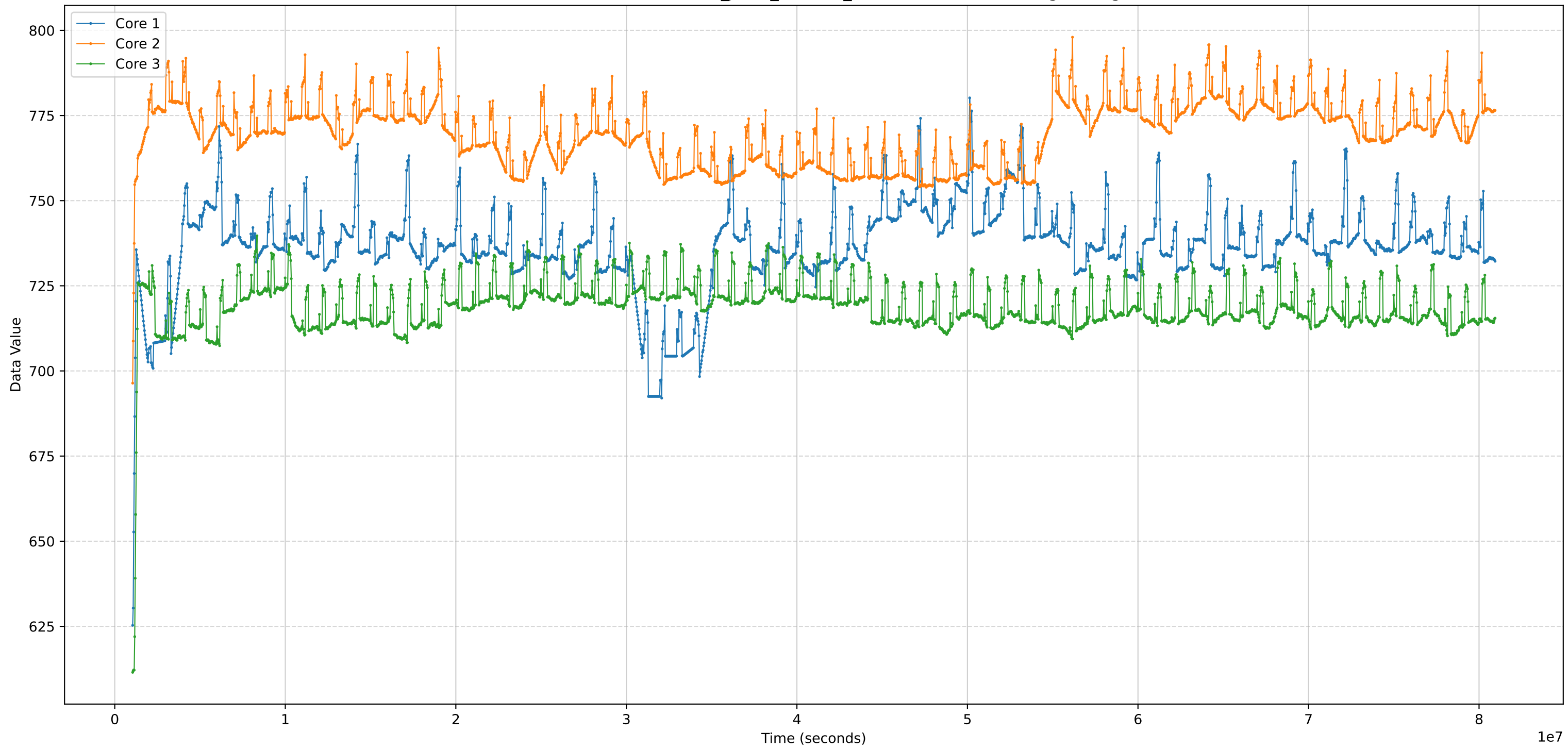
Benchmark Data - BRANCH_JUMP_TARGET_MISPREDICTION - Moving average
