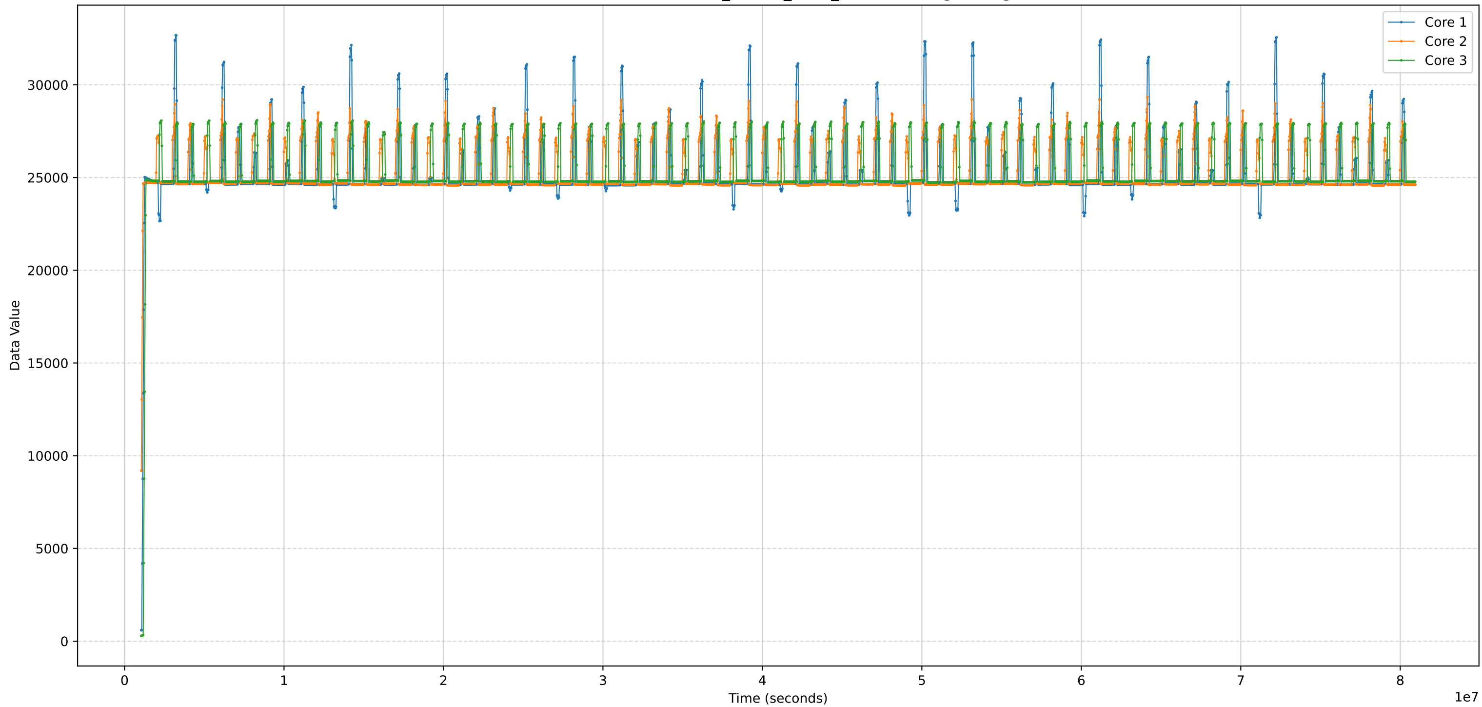
Benchmark Data - DATA_CACHE_DTIM_BUSY - Moving average
