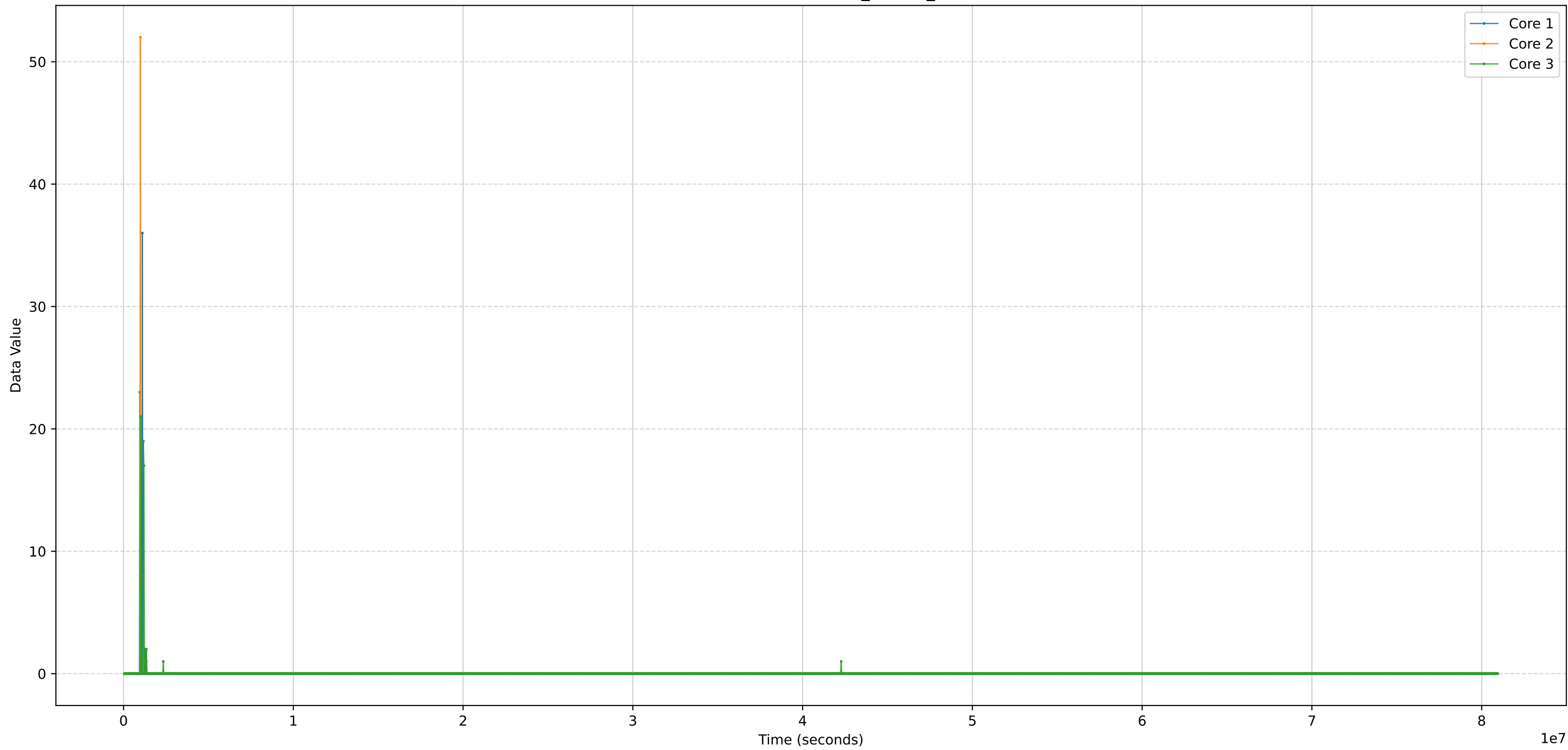
Benchmark Data - INSTRUCTION_CACHE_MISS - Rate
