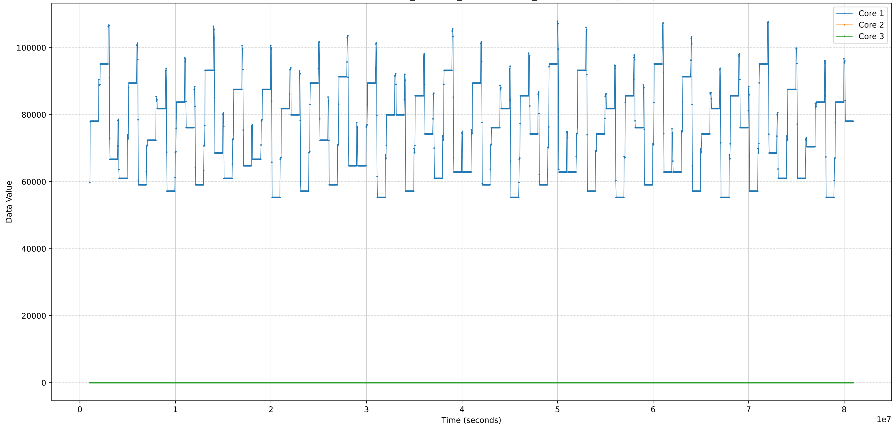
Benchmark Data - INTEGER_DIVISION_INSTRUCTIONS_RETIRED - Moving average
