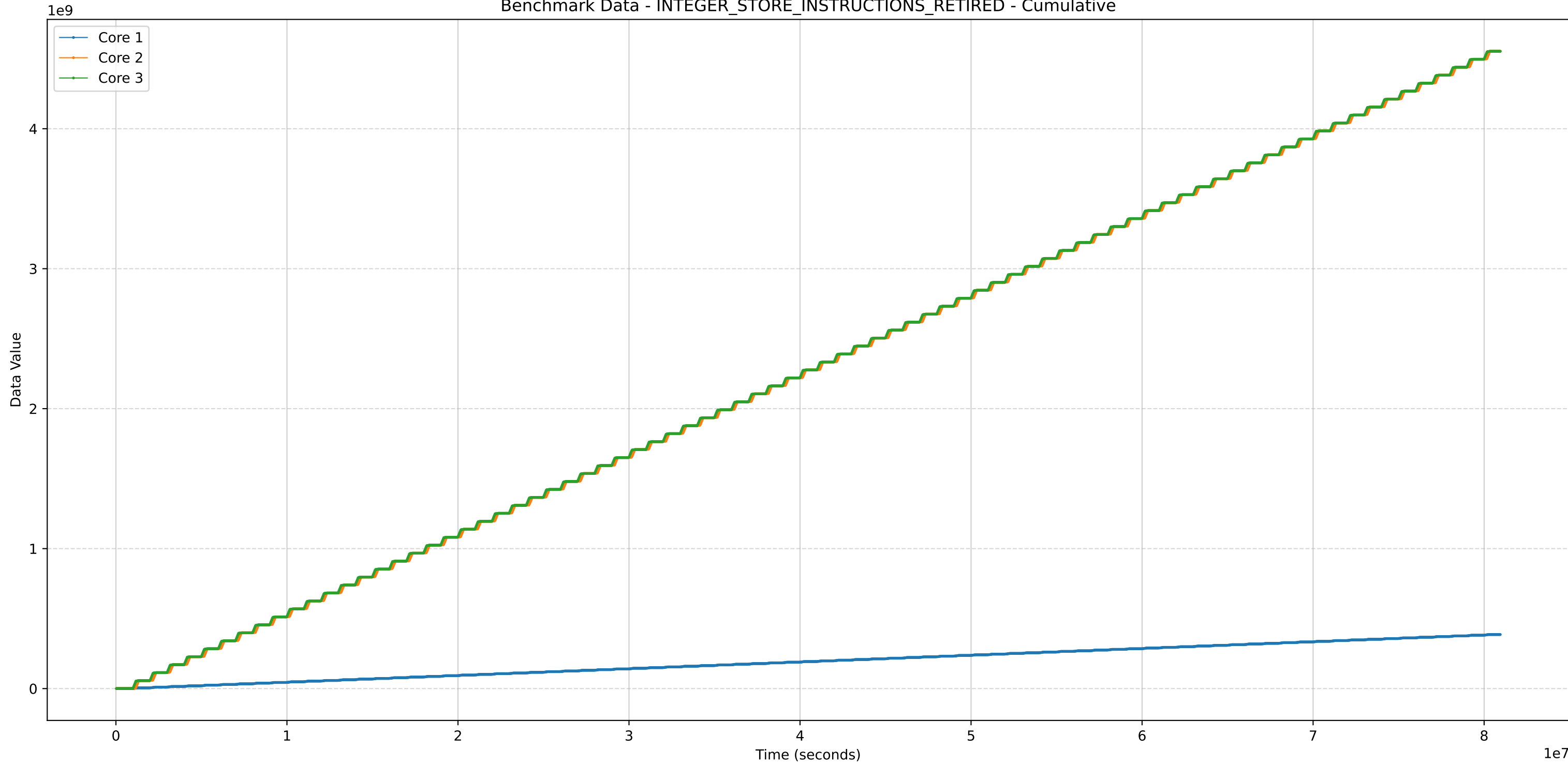
Benchmark Data - INTEGER_STORE_INSTRUCTIONS_RETIRED - Cumulative
