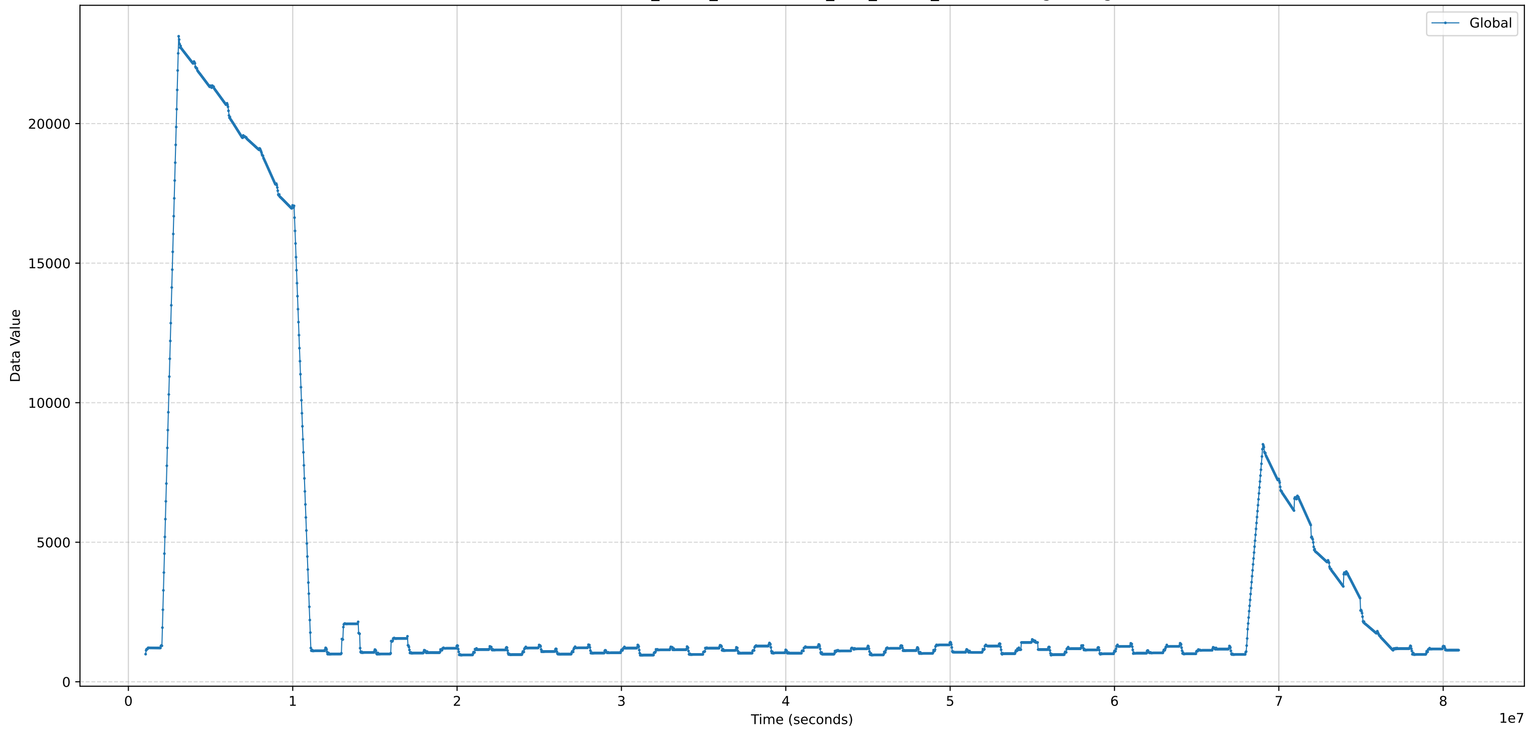
Benchmark Data - L2_INNER_PROBEBLOCK_TON_STORE_MISS - Moving average
