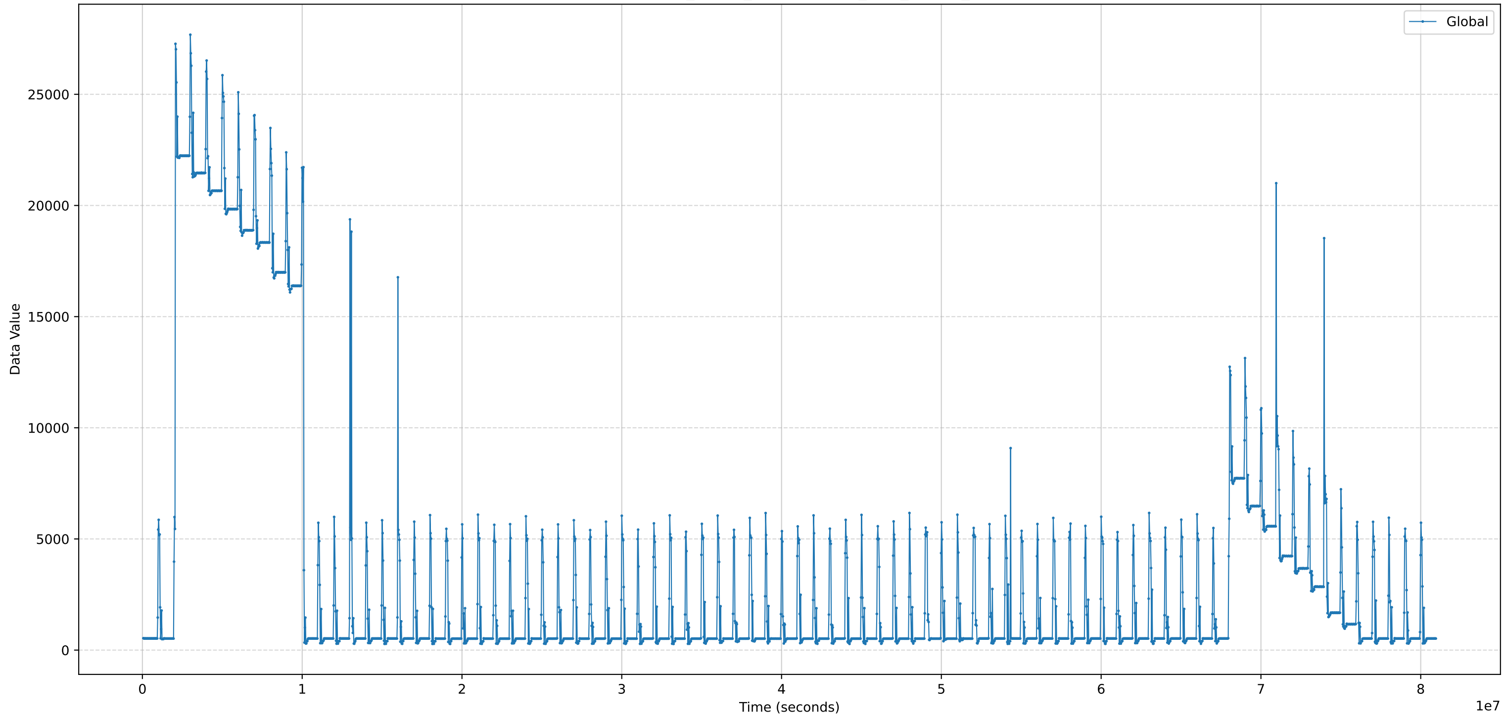
Benchmark Data - L2_INNER_PROBEBLOCK_TON_STORE_MISS - Rate
