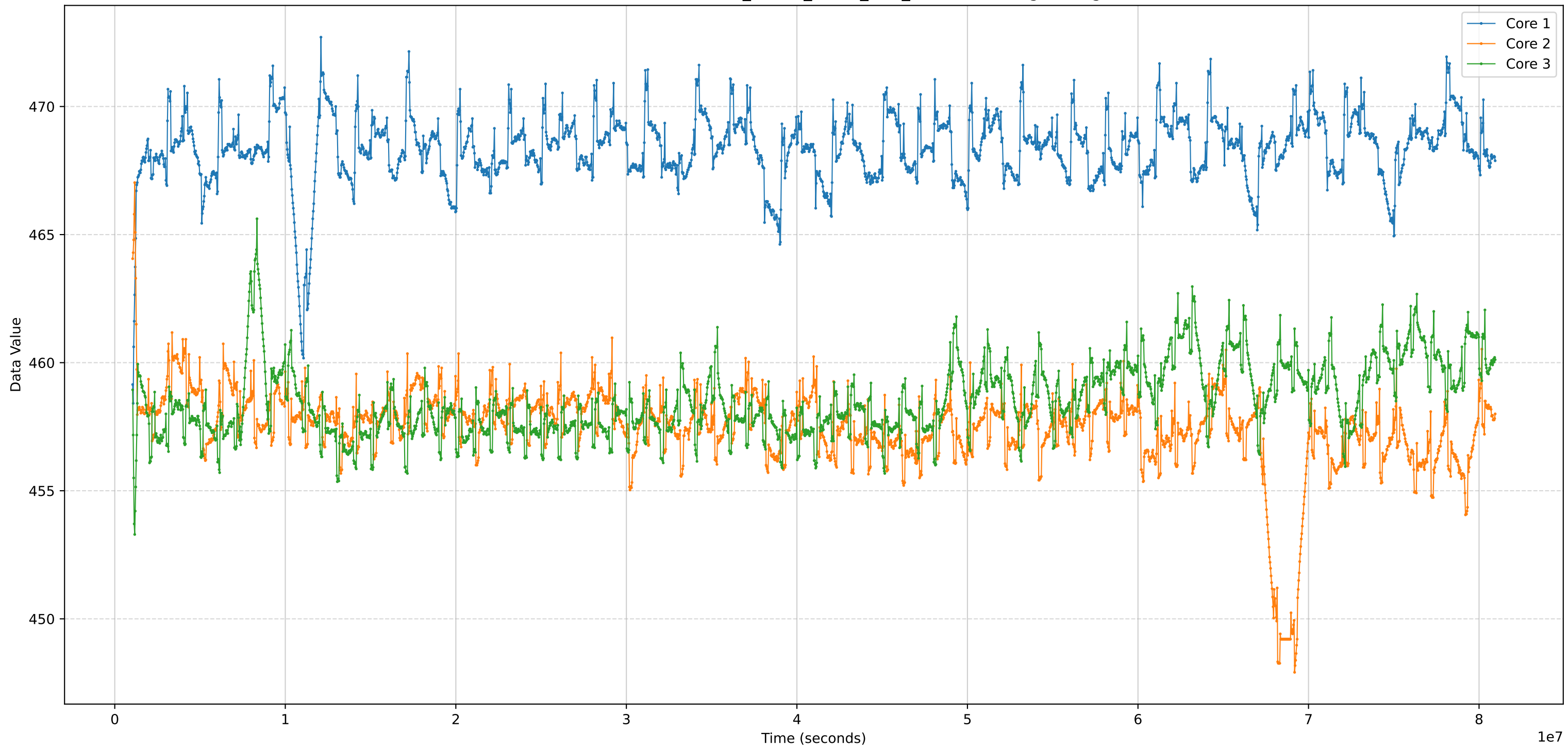
Benchmark Data - PIPELINE_FLUSH_FROM_CSR_WRITE - Moving average
