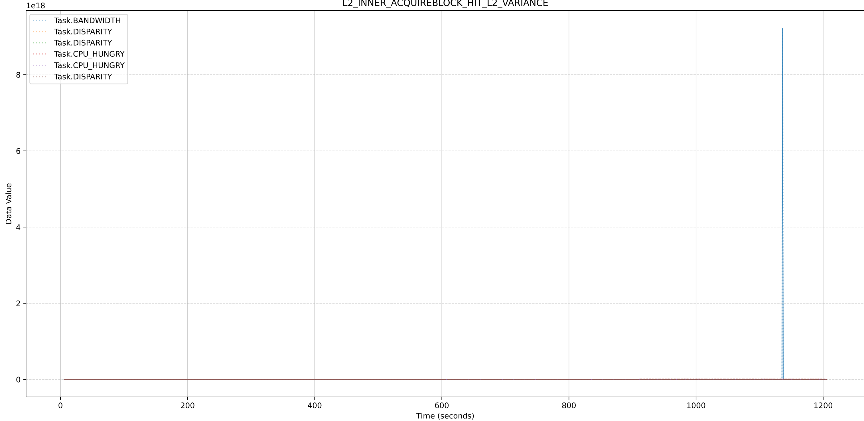
L2_INNER_ACQUIREBLOCK_HIT_L2_VARIANCE
