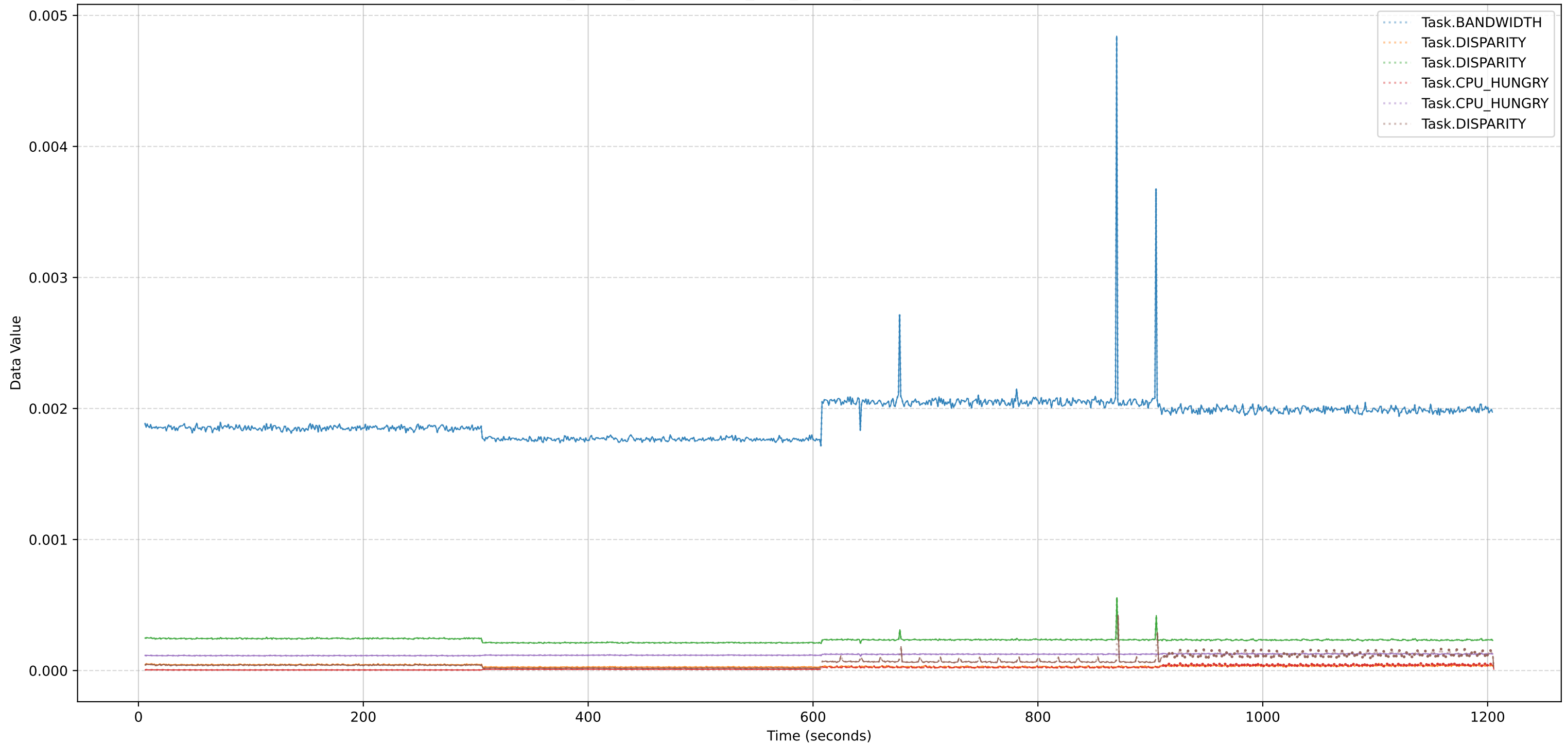
L2_INNER_PROBEBLOCK_TON_STORE_MISS per Instruction Retired
