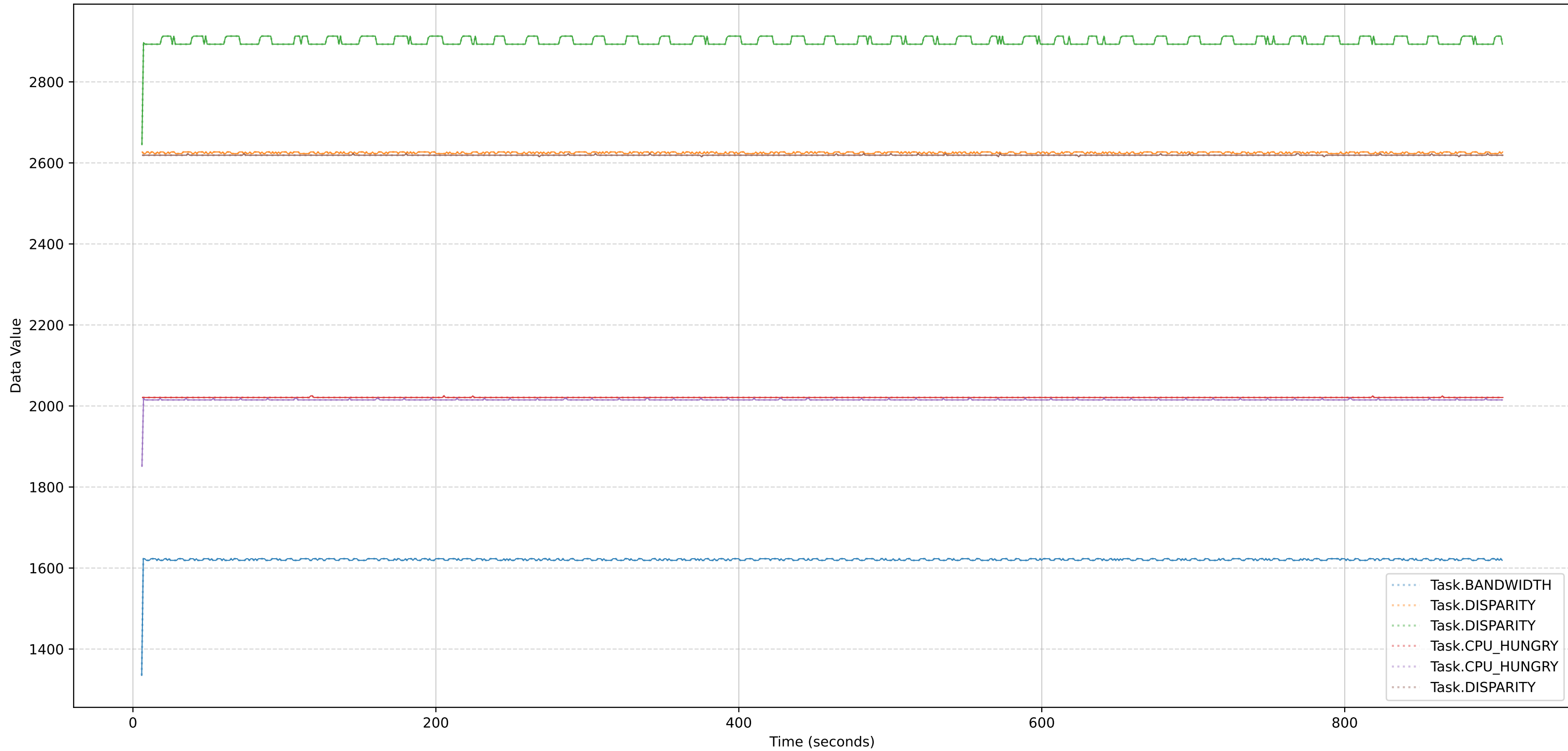
JALR_INSTRUCTIONS_RETIRED
