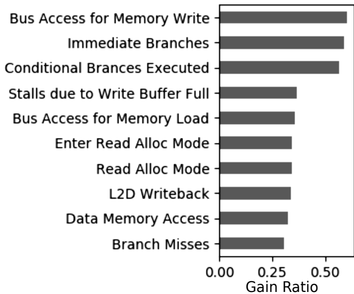
Information Gain Ratio
