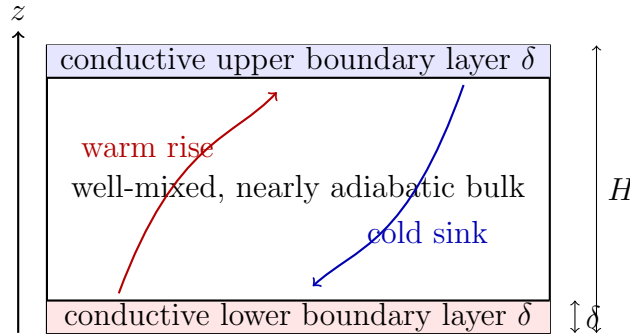
Figure 1: Efficient convection leaves most of the layer close to an adiabatic, well-mixed state. The imposed temperature drop is concentrated in thin conductive boundary layers of thickness \delta .
