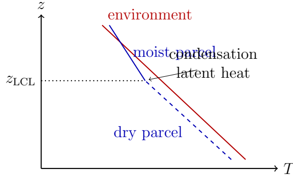
Figure 2: A rising parcel cools along a dry adiabat until it reaches the lifting condensation level z_{\text{LCL}} . Above that height, condensation releases latent heat and the parcel follows a shallower moist adiabat.
