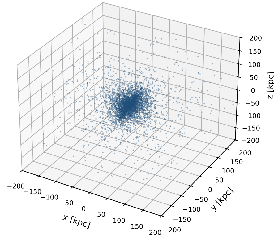
t = 20.0 Gyr (N = 4822, 6.7% outside frame)
