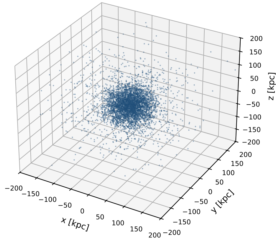
t = 15.0 Gyr (N = 4869, 4.5% outside frame)
