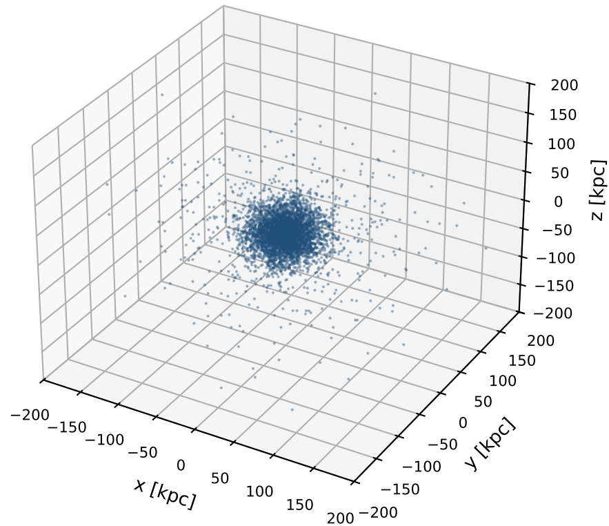
t = 10.0 Gyr (N = 4930, 5.3% outside frame)
