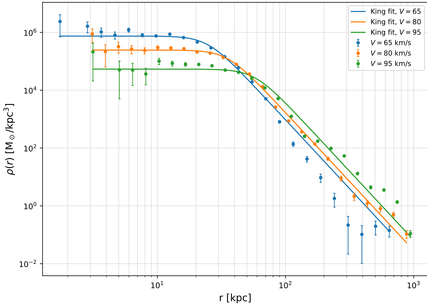
Final density profiles + King fits
