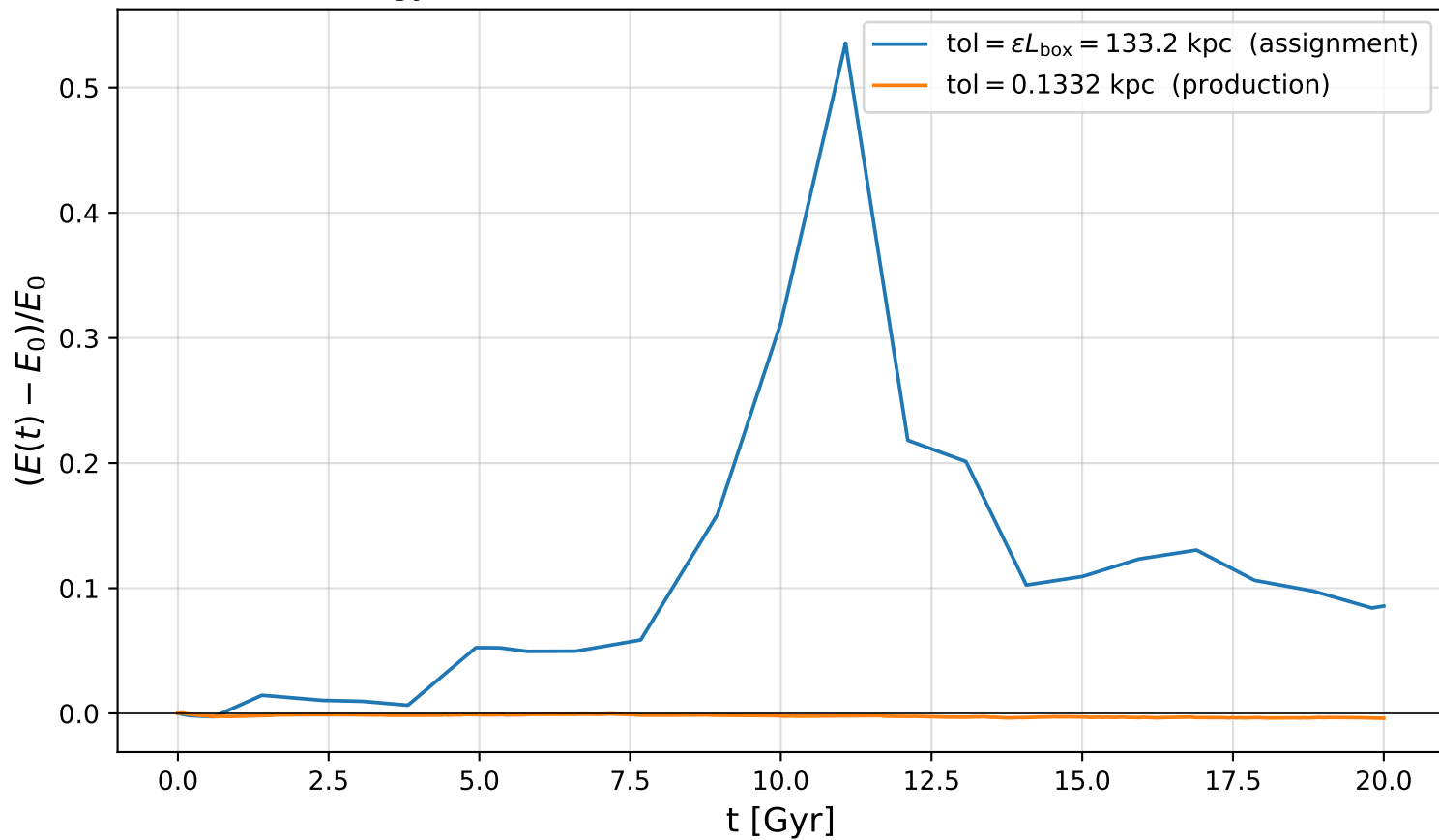
Energy conservation versus RK4 tolerance (V=80 km/s)
