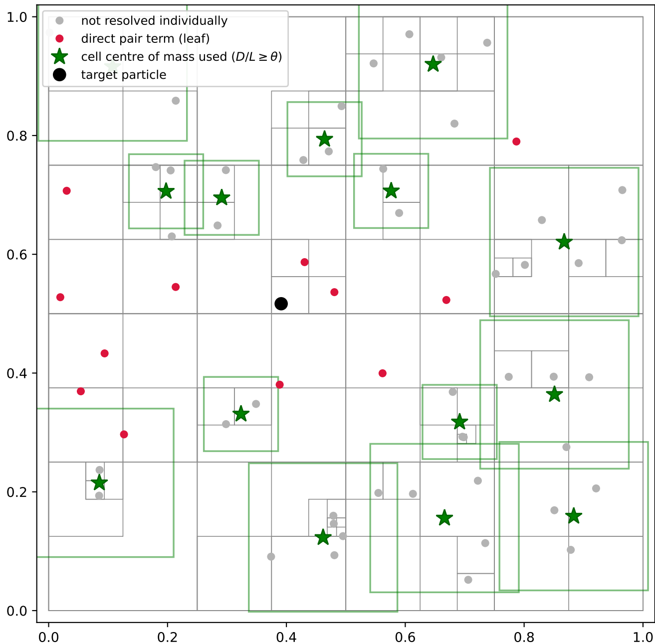
Tree subdivision and force terms for one particle ( N = 60 , \theta = 1 )
