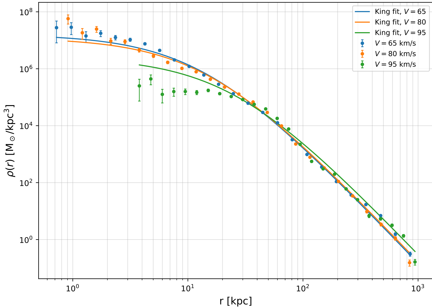
Final density profiles + King fits
