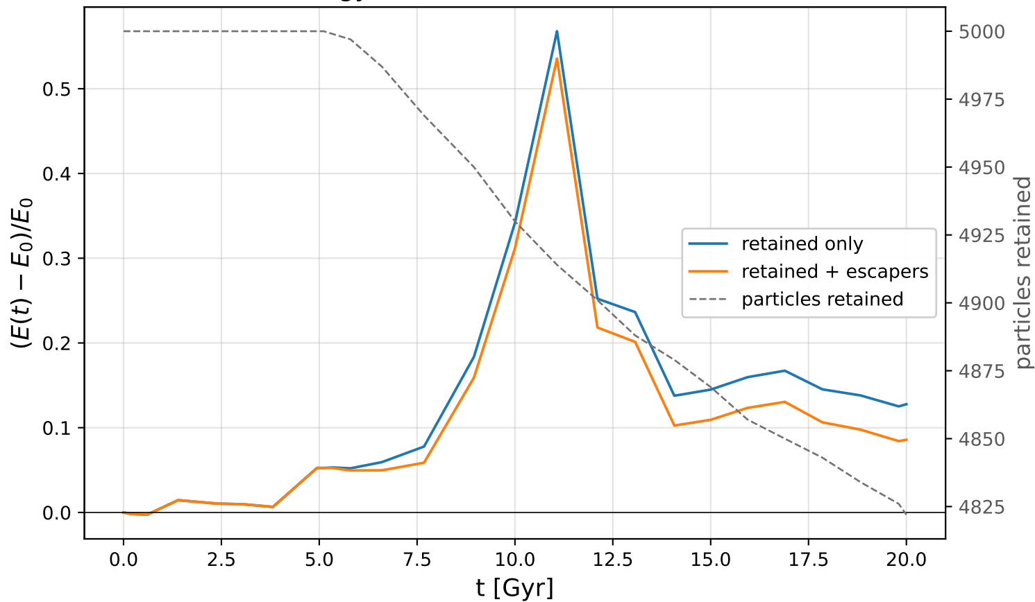
Energy conservation (V=80.0 km/s)
