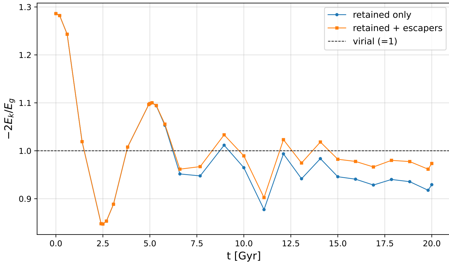
Virial ratio ( V=80.0 km/s)
