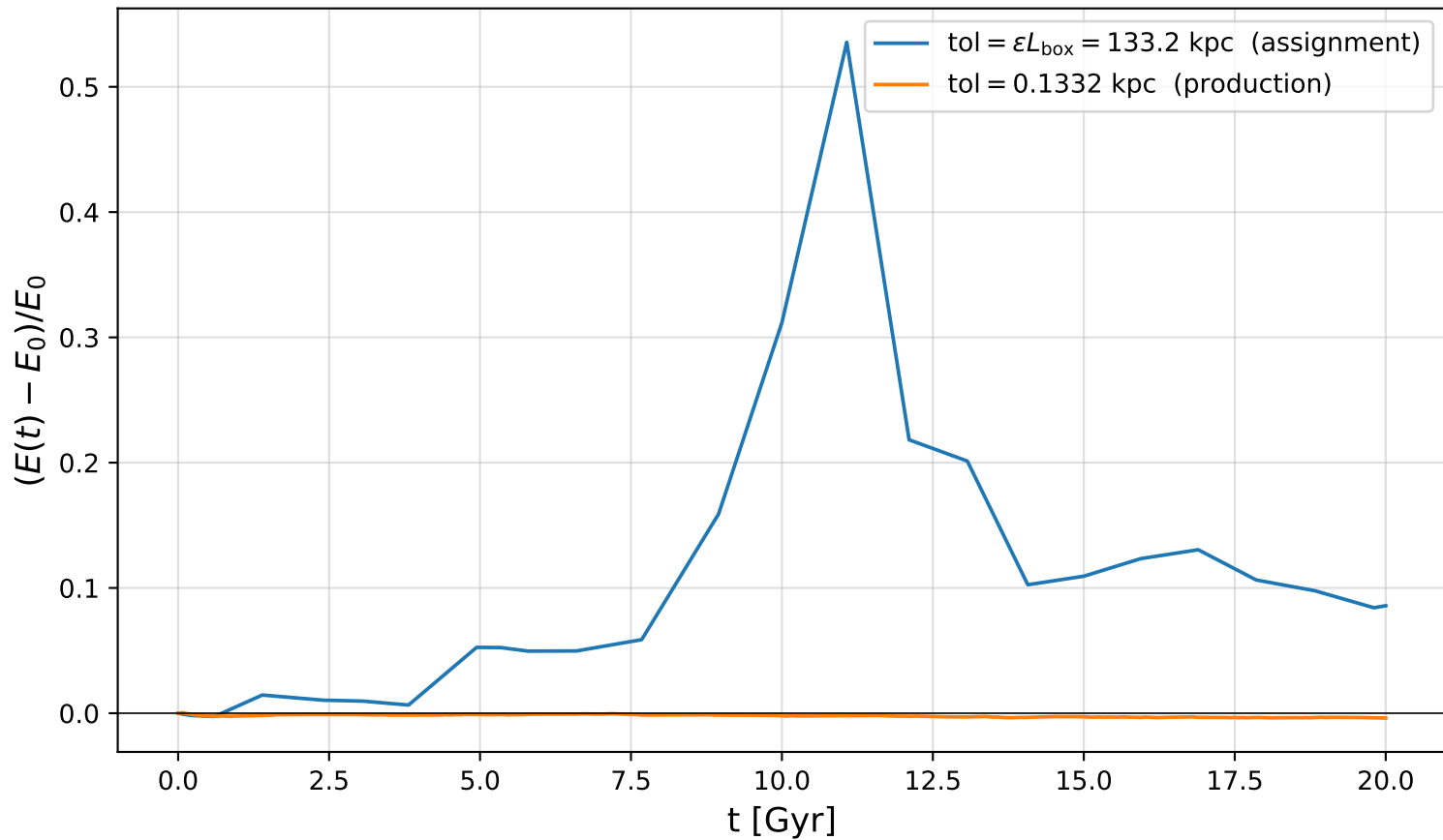
Energy conservation versus RK4 tolerance ( V=80 km/s)
