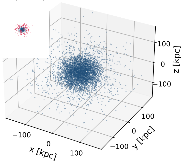
t = 10.0 Gyr N = 4932 , 5.6% only in the inset
