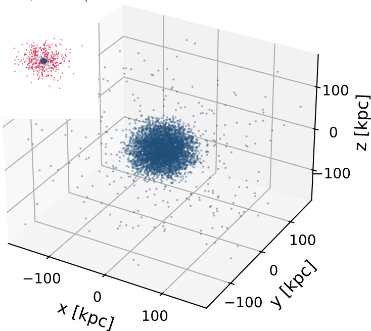
t = 15.0 Gyr N = 4872 , 3.9% only in the inset
