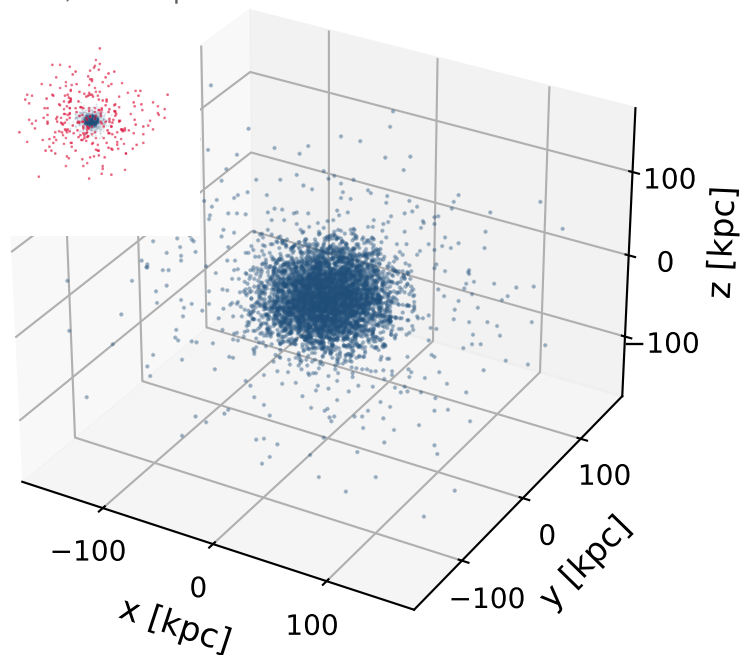
t = 20.0 Gyr N = 4833 , 3.1% only in the inset
