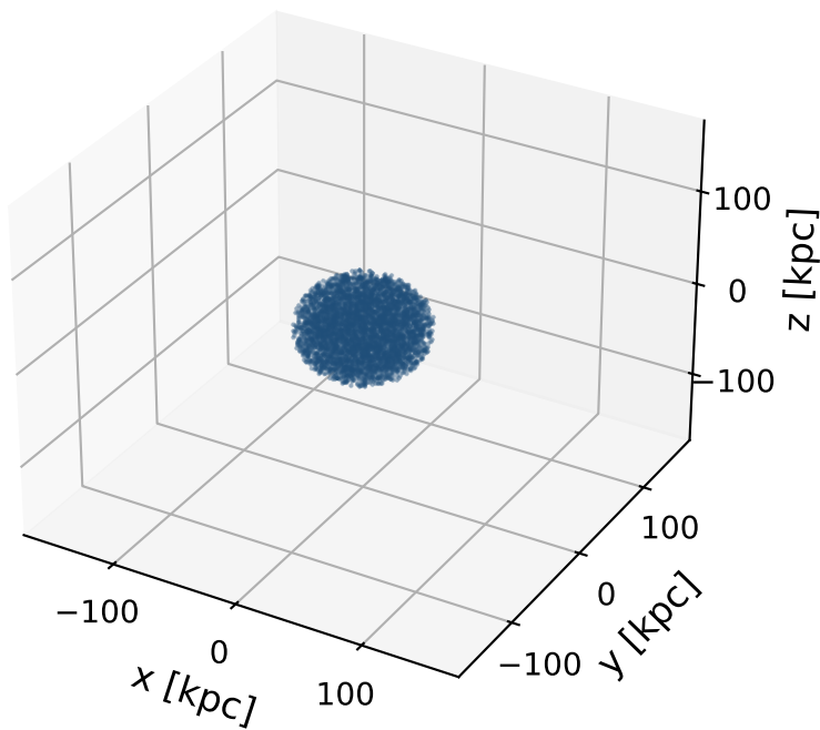
t = 5.0 Gyr N = 5000 , 7.2% only in the inset
