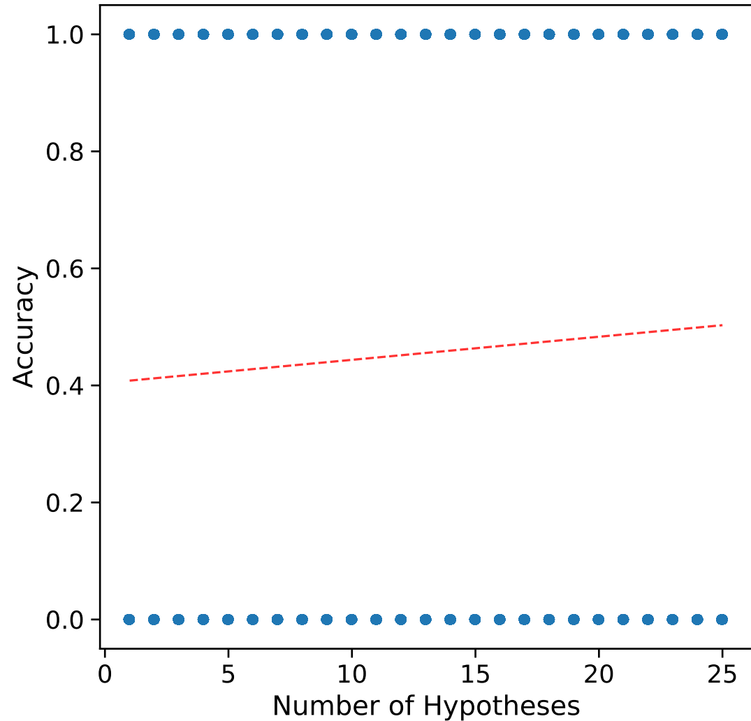
Correlation: 0.057
