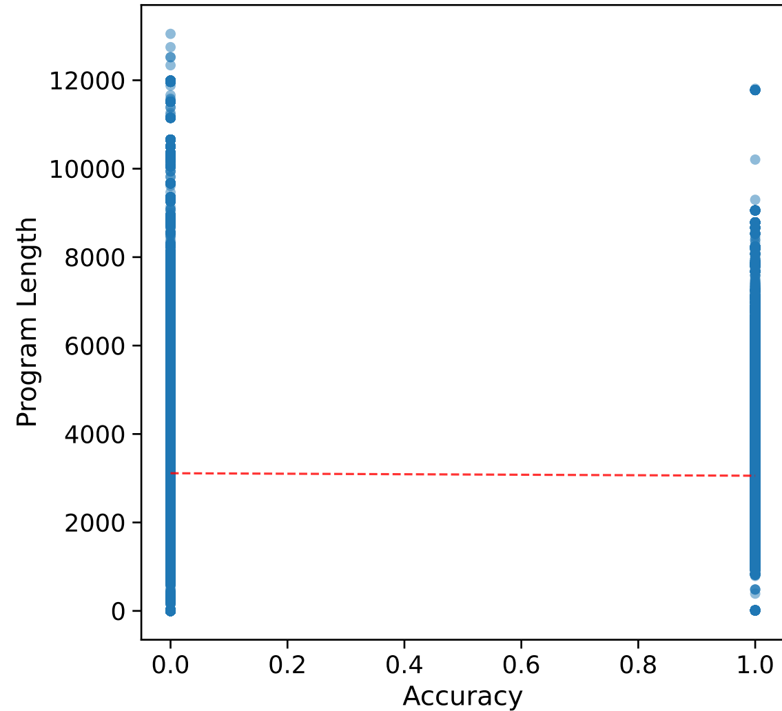
Correlation: -0.019
