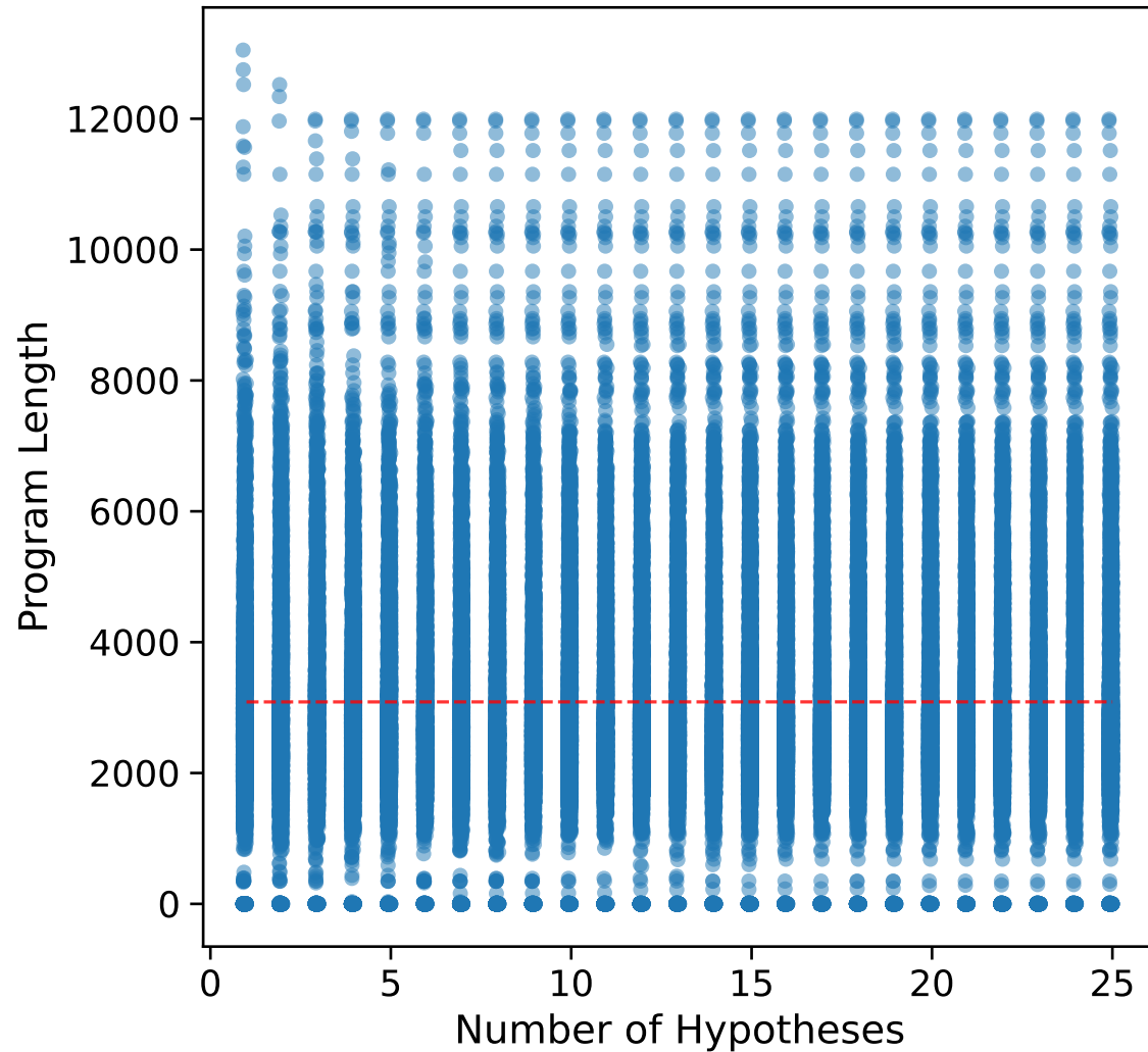
Correlation: 0.000
