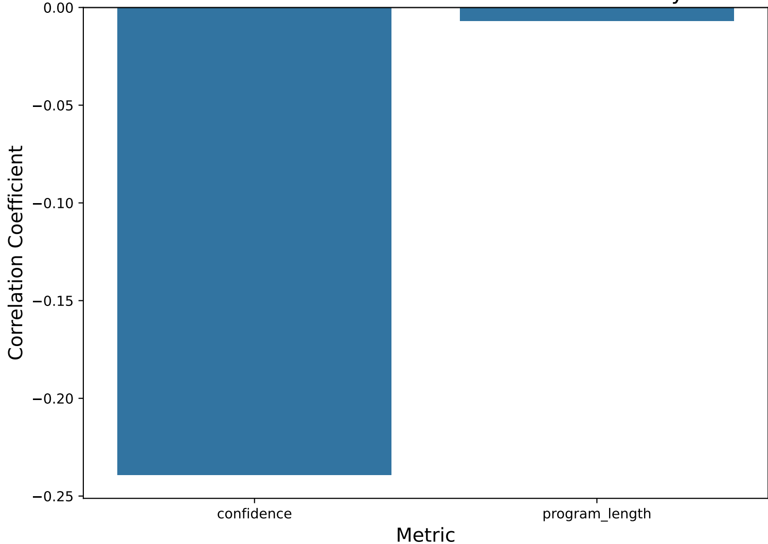
Correlation between FSM Metrics and Accuracy
