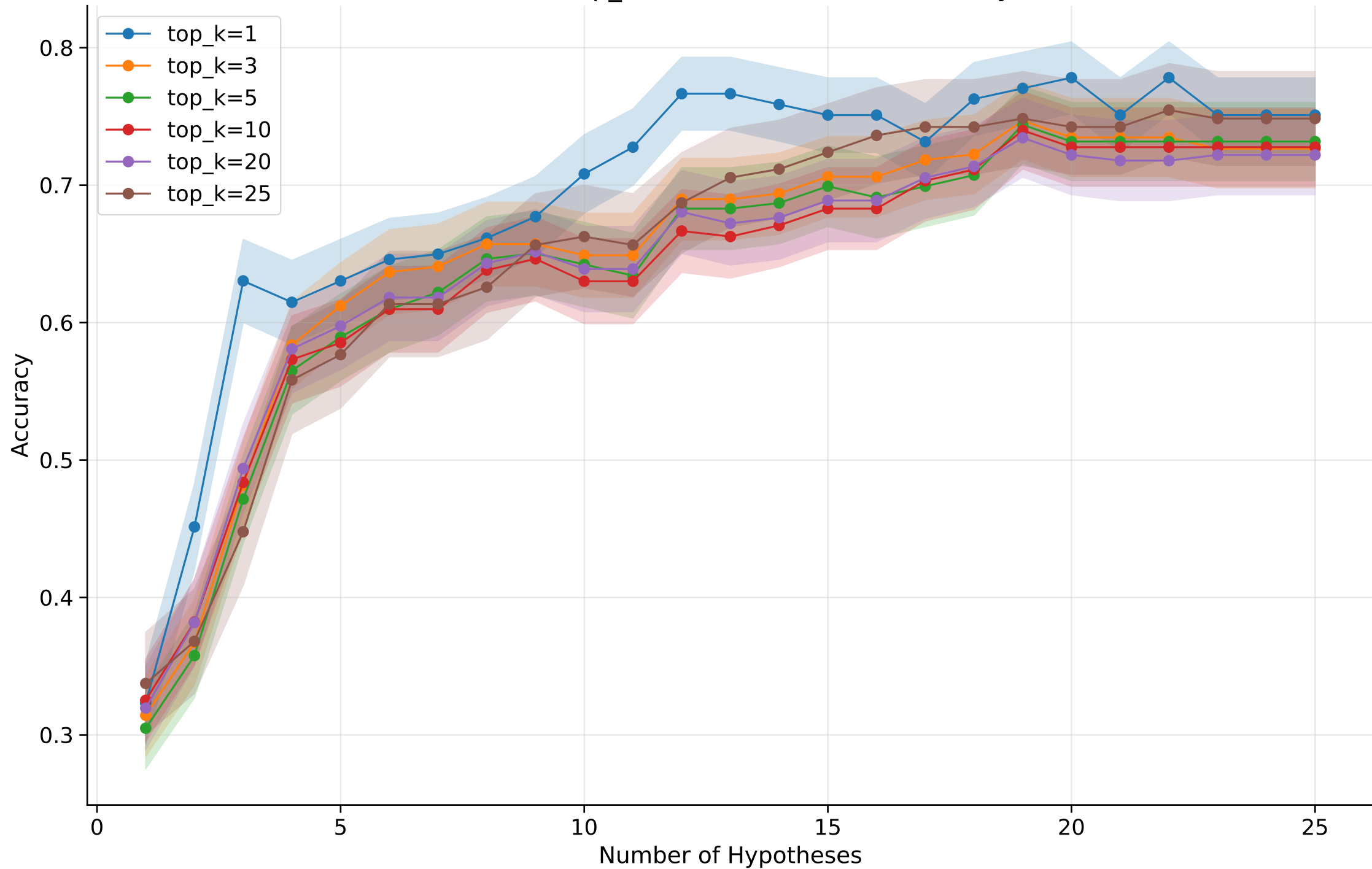
Effect of top_k Parameter on FSM Accuracy
