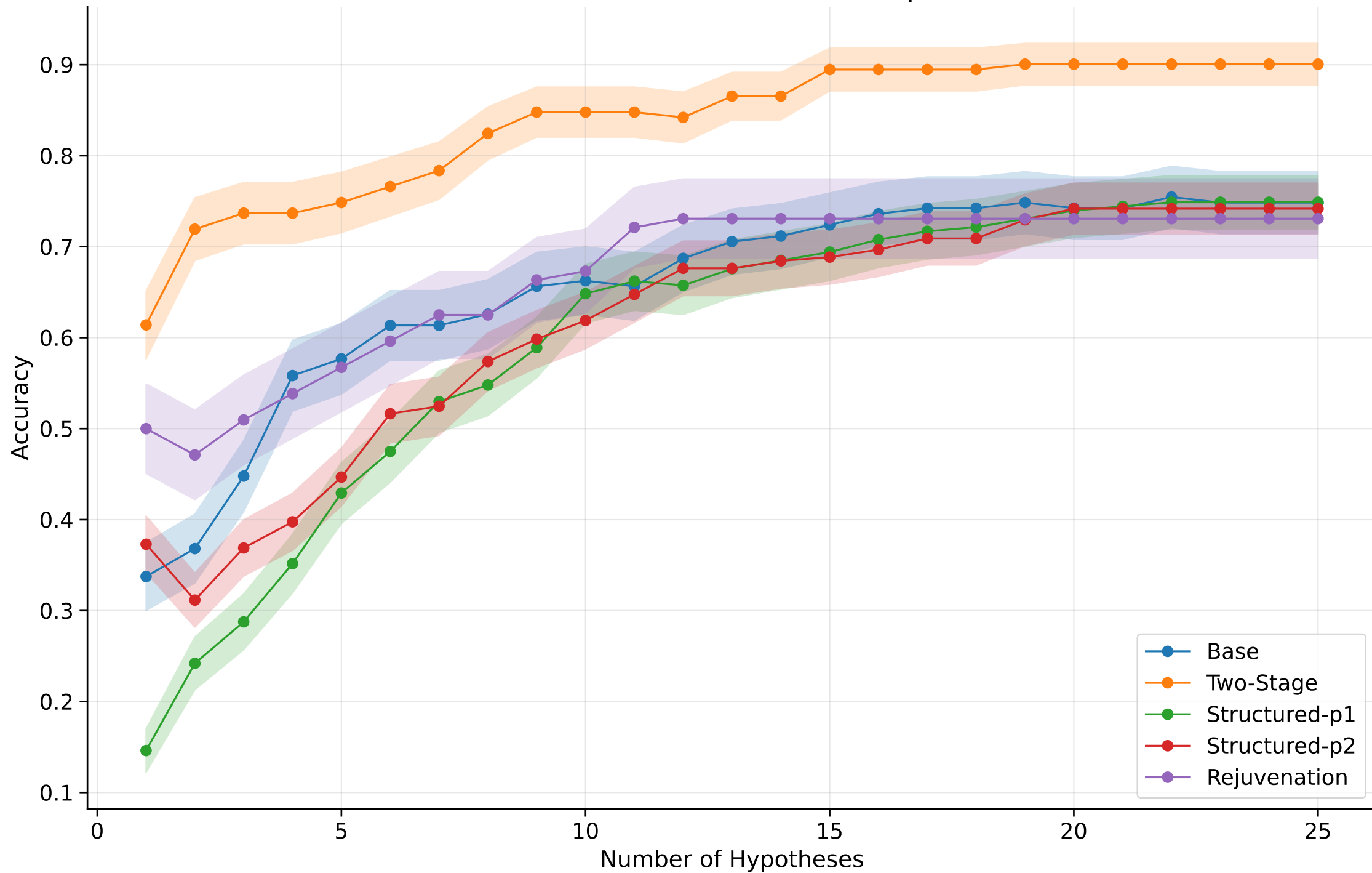
Grid Dataset: Ablation of FSM Components
