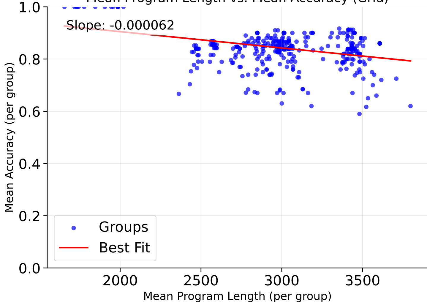
Mean Program Length vs. Mean Accuracy (Grid)
