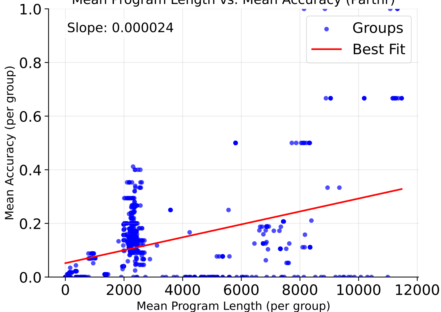
Mean Program Length vs. Mean Accuracy (Partnr)
