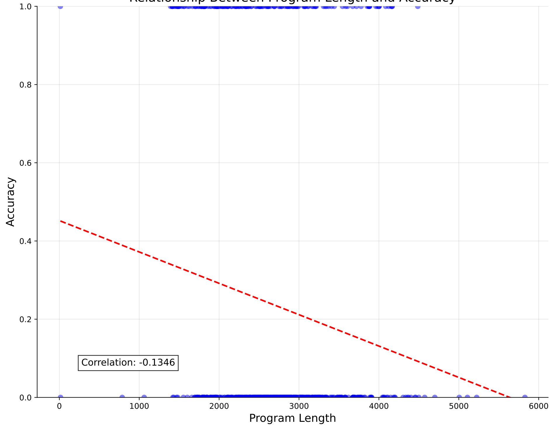
Relationship Between Program Length and Accuracy
