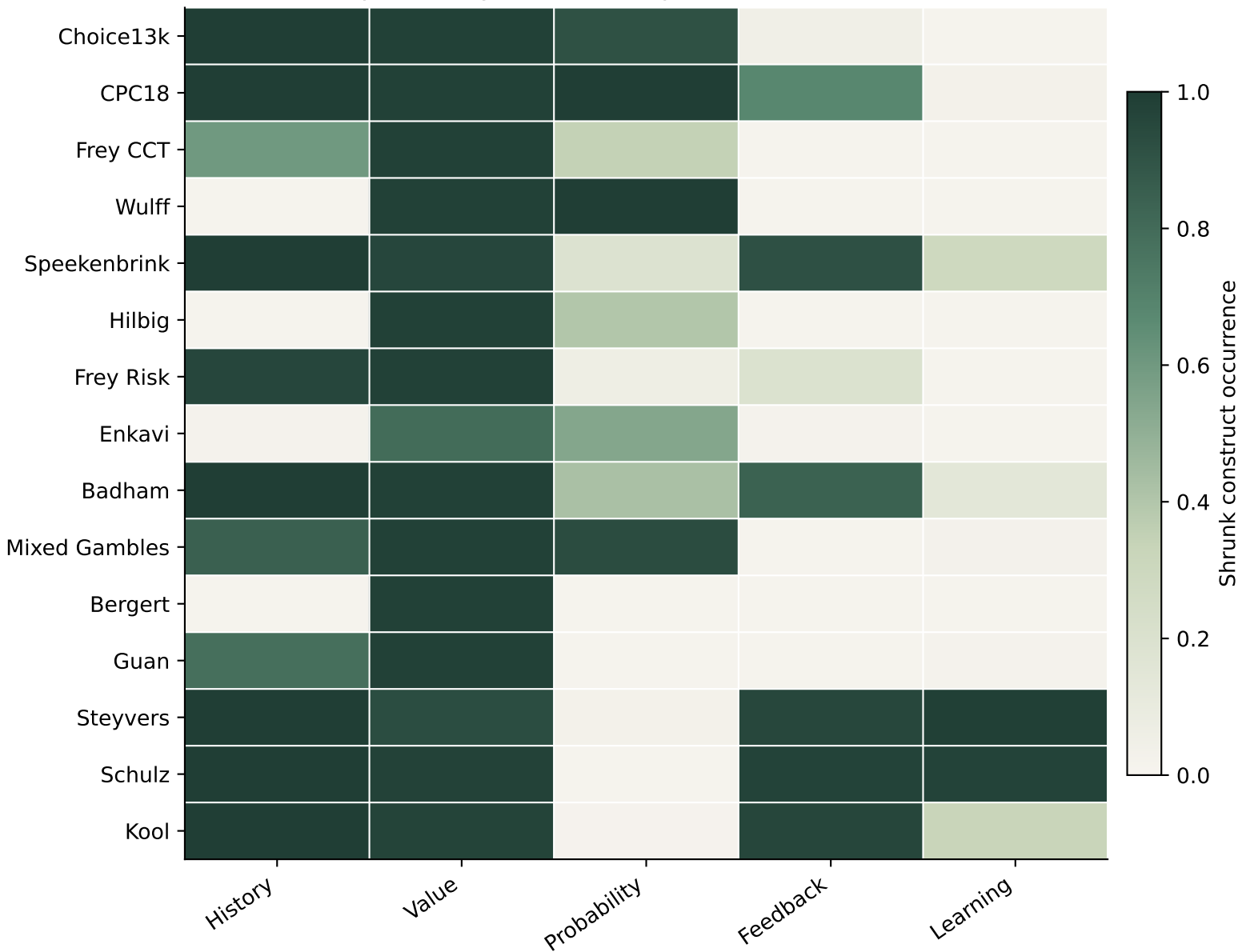
Empirical-Bayes construct profiles (five constructs)
