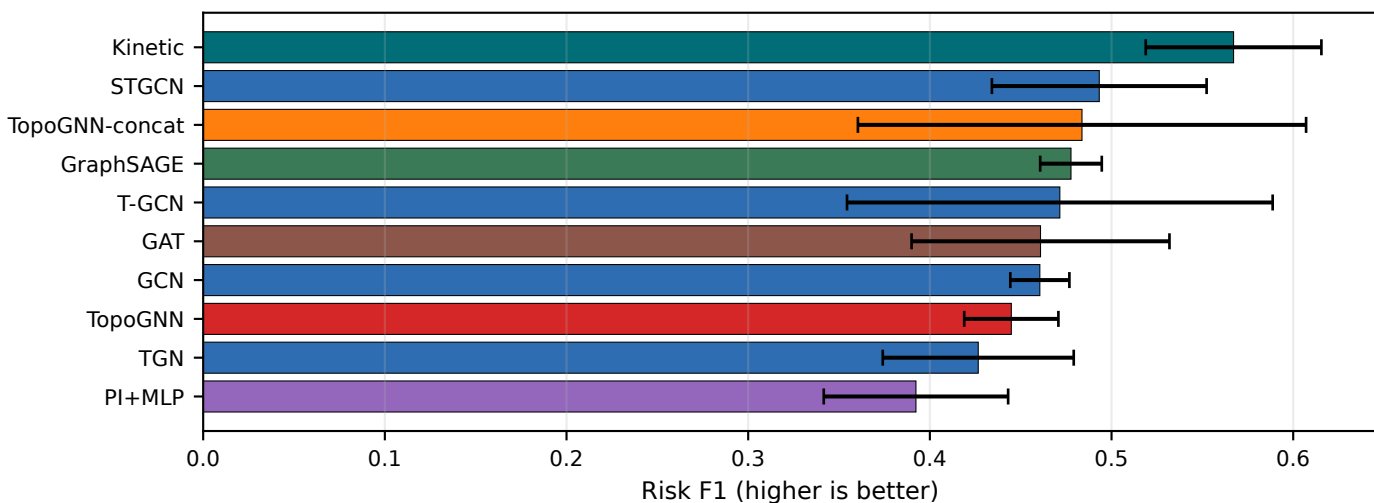
Risk F1 with 95% CI
