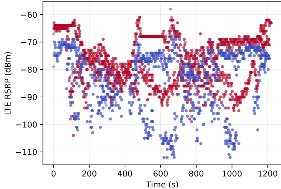
Measured aerial LTE link state
