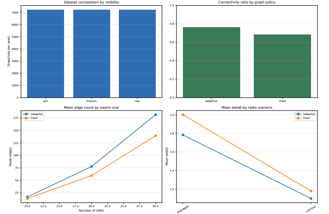
Figure 3: Dataset and graph-construction overview for the calibrated evaluation. The panels summarise mobility composition, fixed/adaptive connectivity, edge counts by swarm size, and mean \beta_0 under the nominal and degraded radio scenarios.
