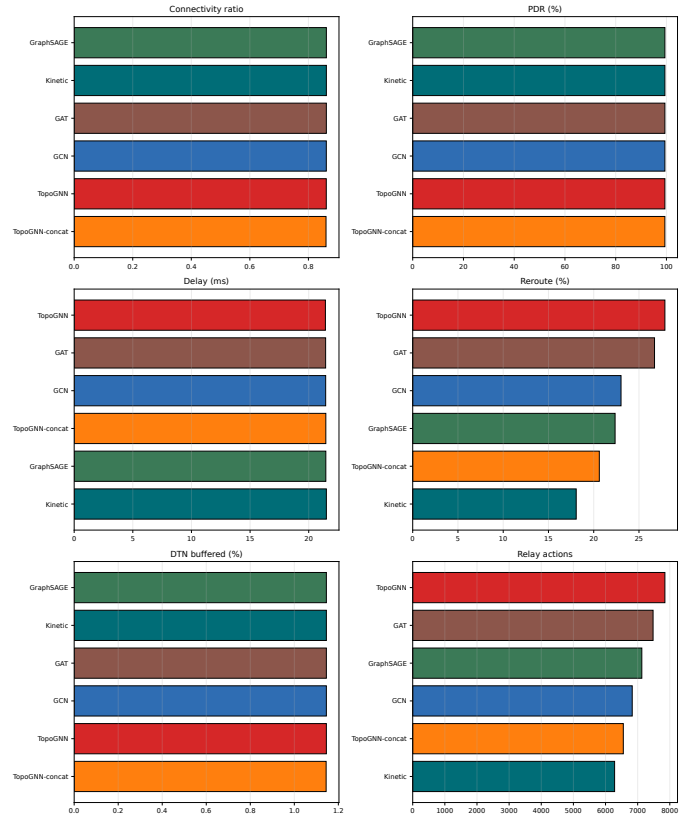
Figure 13: Extended controller-level metrics, including connectivity, PDR, delay, proactive rerouting, DTN buffering, and relay actions, computed on the physical-radio snapshot graph. Kinetic-TopoGuard matches the strongest evaluated GNN controller on connectivity and PDR while using a more conservative reroute/relay policy.
