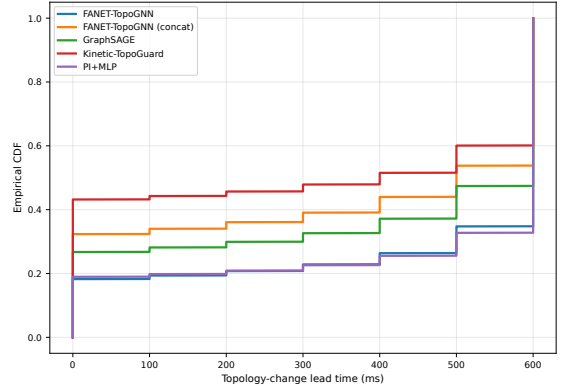
Figure 9: Empirical CDF of topology-change lead time. The curves are truncated by the six-step horizon, which motivates the cautious interpretation of lead-time differences.
