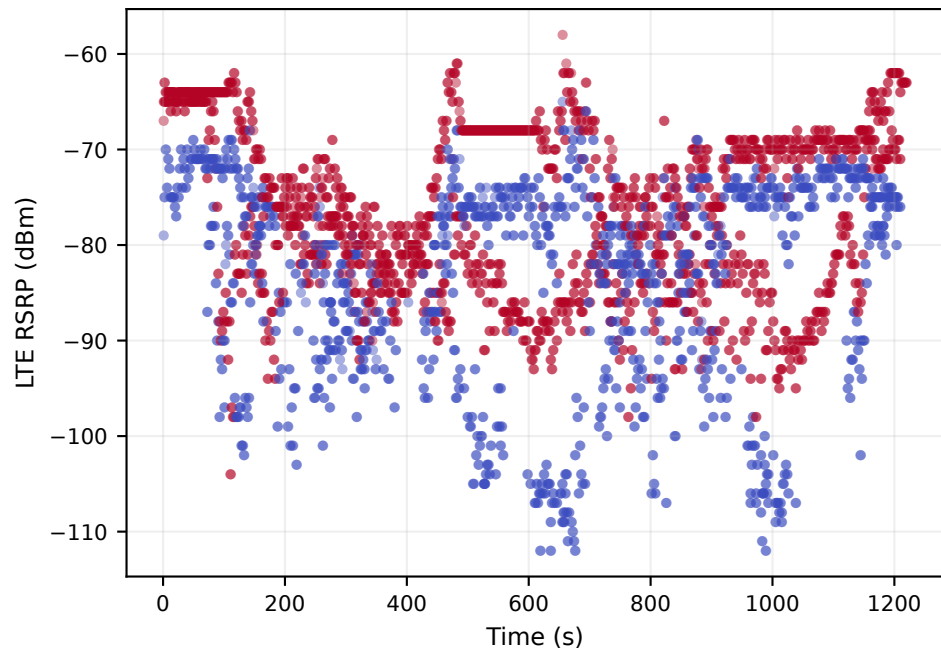
Measured aerial LTE link state
